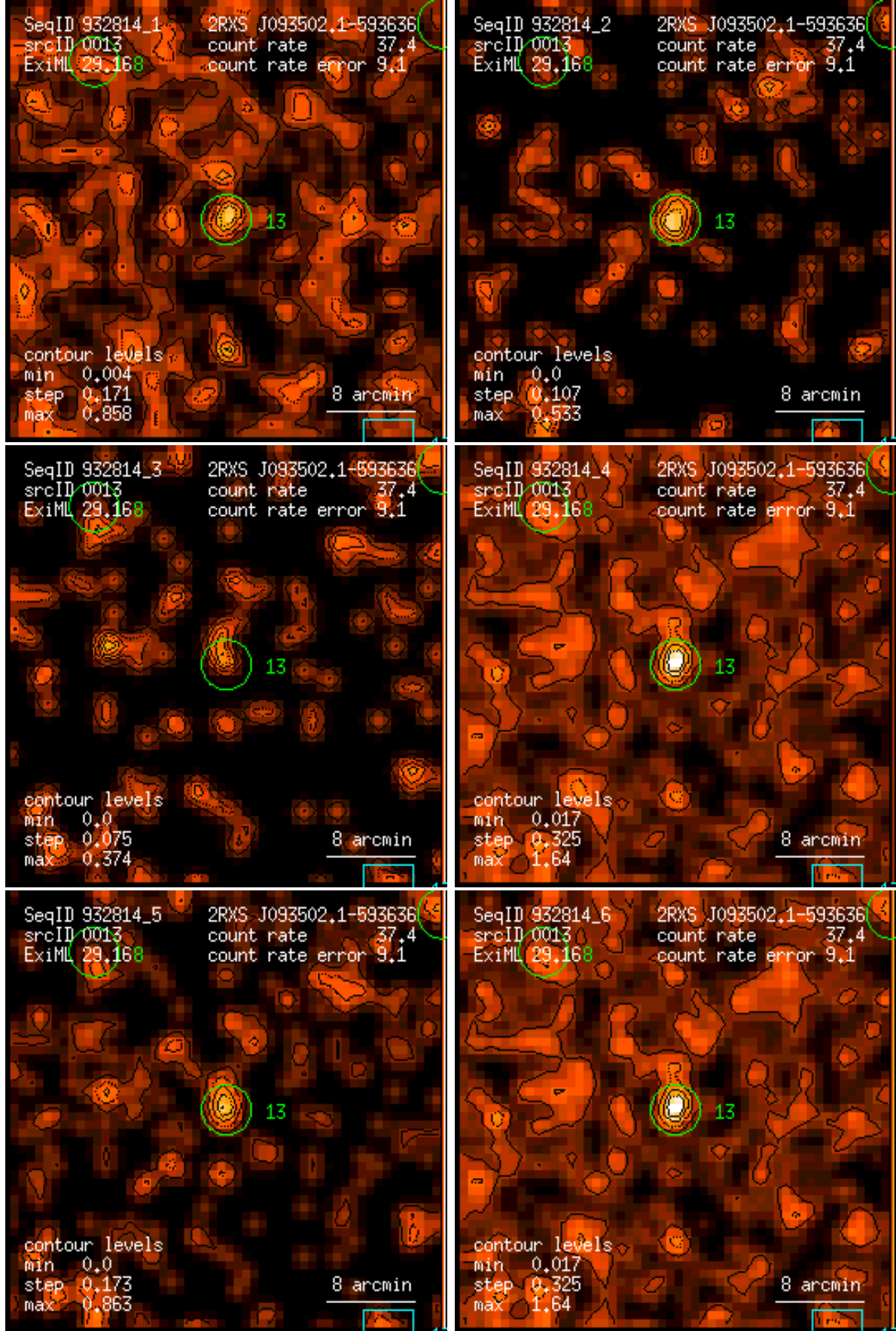
Figure 13: RASS 932814: detection 0013: band rate images, Gaussian filter: (1) PSPC channels 11 – 41, (2) 52 – 90, (3) 91 – 201, (4) 11 – 235, (5) 52 – 201, (6) 11 – 201. Broad band rates in counts/ks. Band rate contour levels in counts/ks/arcmin 2 .
