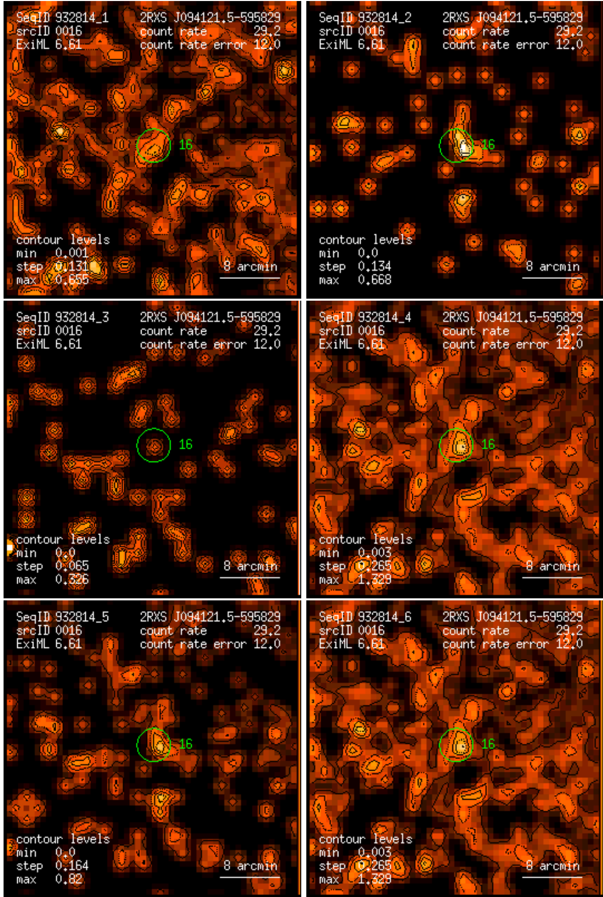
Figure 16: RASS 932814: detection 0016: band rate images, Gaussian filter: (1) PSPC channels 11 – 41, (2) 52 – 90, (3) 91 – 201, (4) 11 – 235, (5) 52 – 201, (6) 11 – 201. Broad band rates in counts/ks. Band rate contour levels in counts/ks/arcmin 2 .
