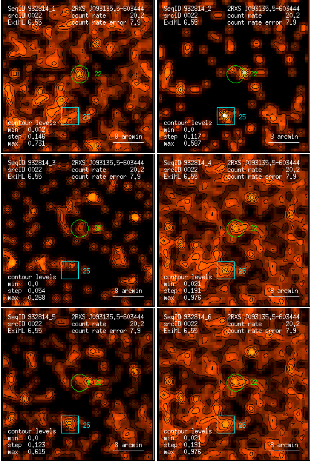
Figure 22: RASS 932814: detection 0022: band rate images, Gaussian filter: (1) PSPC channels 11 – 41, (2) 52 – 90, (3) 91 – 201, (4) 11 – 235, (5) 52 – 201, (6) 11 – 201. Broad band rates in counts/ks. Band rate contour levels in counts/ks/arcmin 2 .
