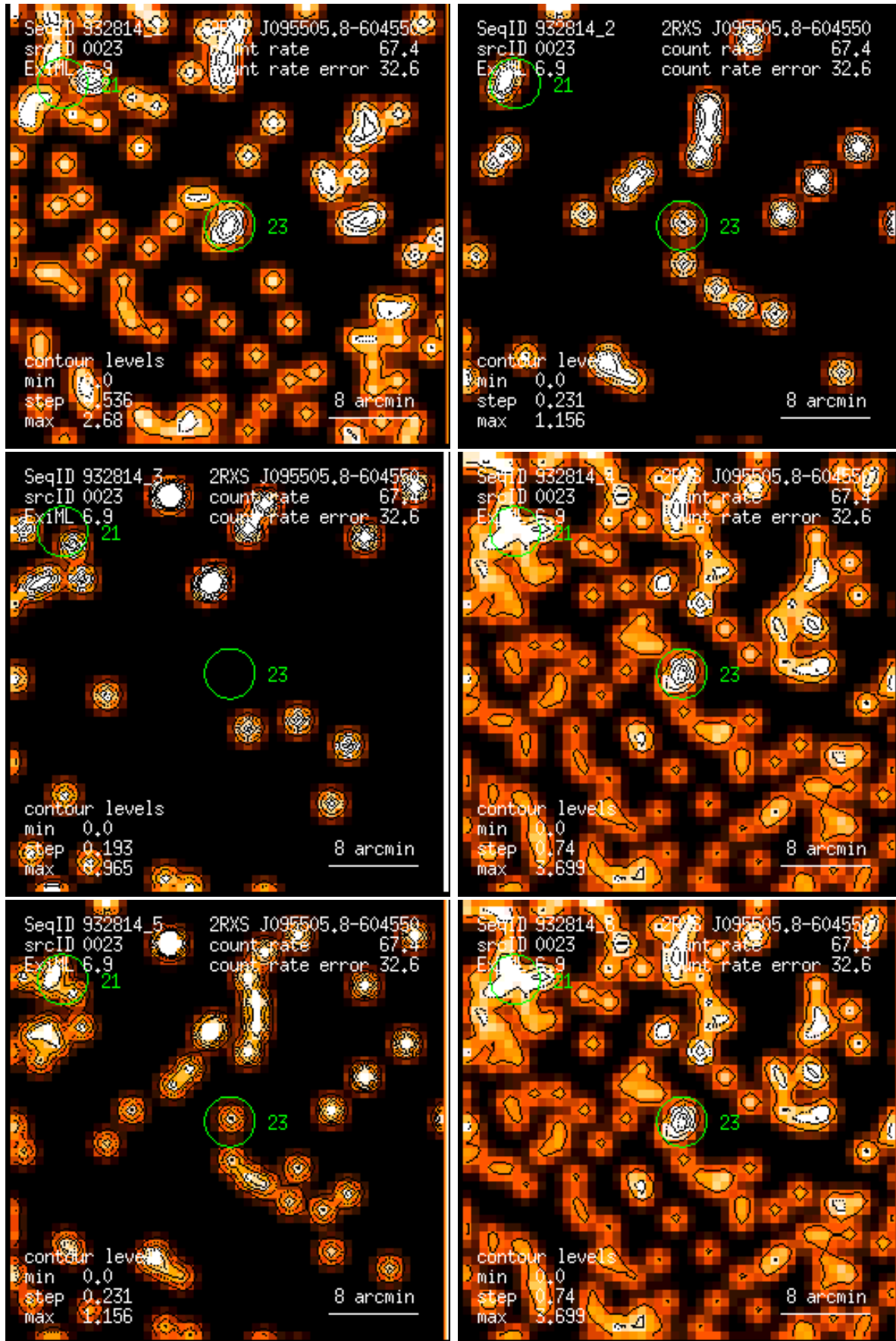
Figure 23: RASS 932814: detection 0023: band rate images, Gaussian filter: (1) PSPC channels 11 – 41, (2) 52 – 90, (3) 91 – 201, (4) 11 – 235, (5) 52 – 201, (6) 11 – 201. Broad band rates in counts/ks. Band rate contour levels in counts/ks/arcmin 2 .
