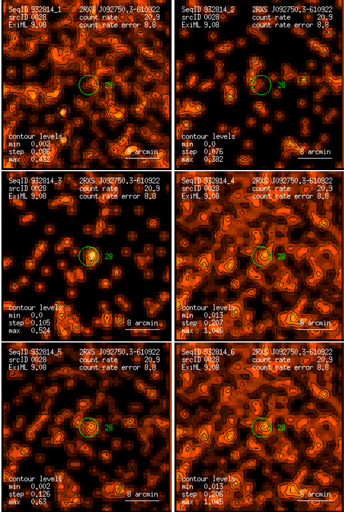
Figure 28: RASS 932814: detection 0028: band rate images, Gaussian filter: (1) PSPC channels 11 – 41, (2) 52 – 90, (3) 91 – 201, (4) 11 – 235, (5) 52 – 201, (6) 11 – 201. Broad band rates in counts/ks. Band rate contour levels in counts/ks/arcmin 2 .
