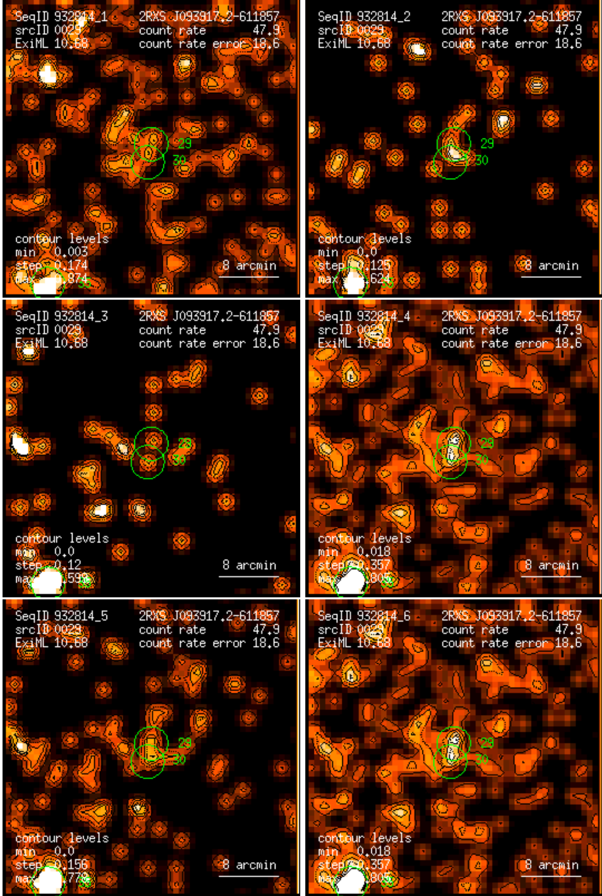
Figure 29: RASS 932814: detection 0029: band rate images, Gaussian filter: (1) PSPC channels 11 – 41, (2) 52 – 90, (3) 91 – 201, (4) 11 – 235, (5) 52 – 201, (6) 11 – 201. Broad band rates in counts/ks. Band rate contour levels in counts/ks/arcmin 2 .
