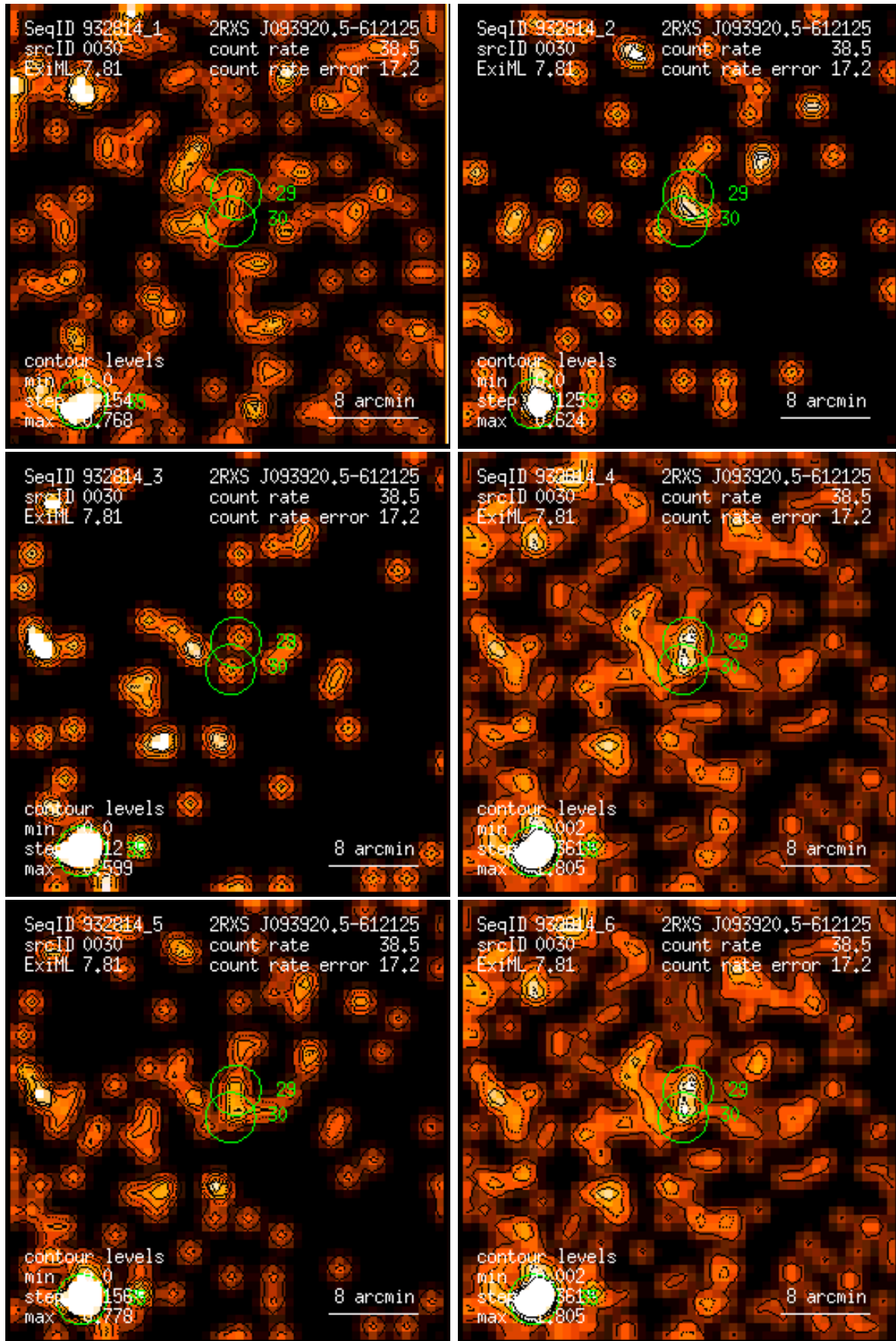
Figure 30: RASS 932814: detection 0030: band rate images, Gaussian filter: (1) PSPC channels 11 – 41, (2) 52 – 90, (3) 91 – 201, (4) 11 – 235, (5) 52 – 201, (6) 11 – 201. Broad band rates in counts/ks. Band rate contour levels in counts/ks/arcmin 2 .
