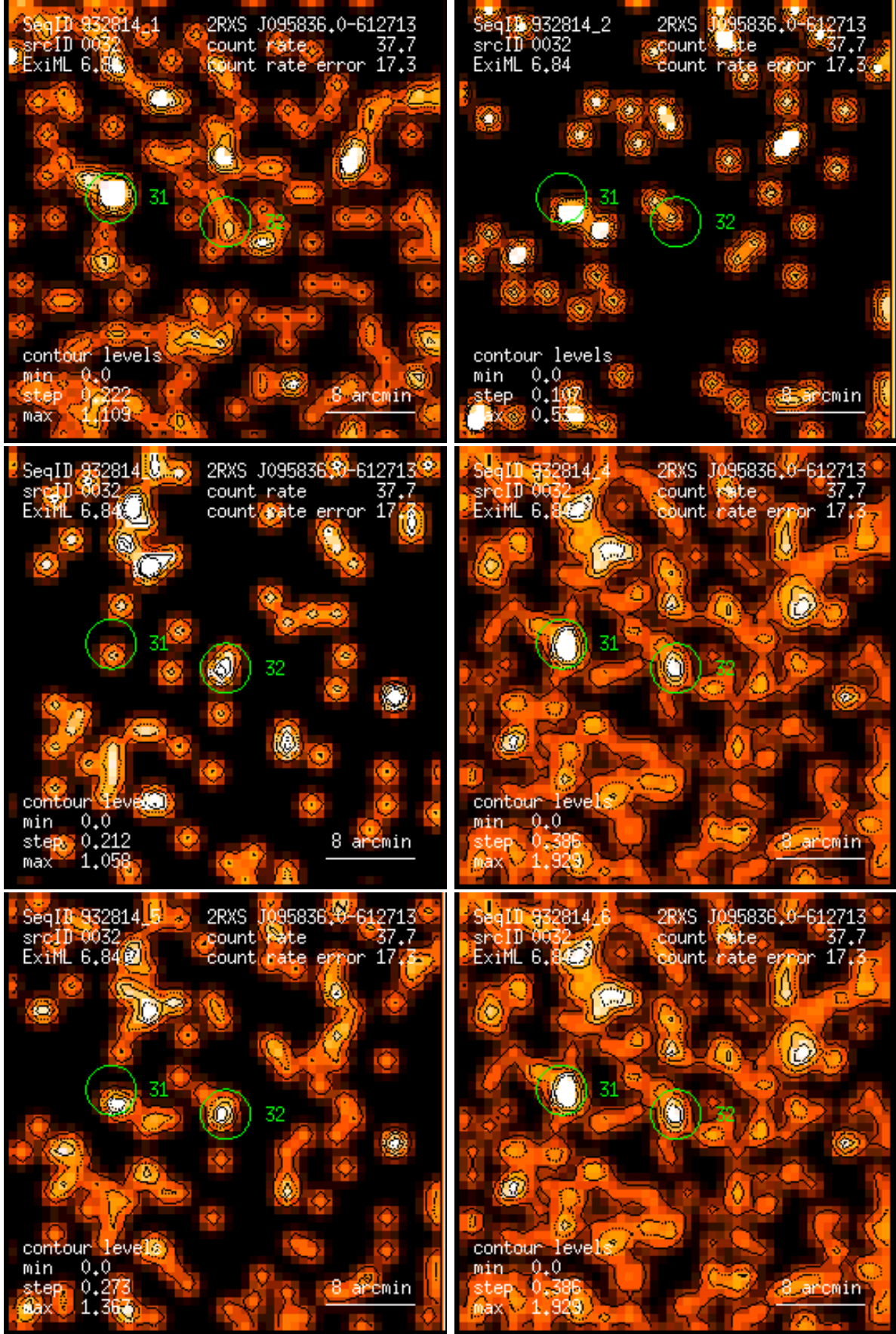
Figure 32: RASS 932814: detection 0032: band rate images, Gaussian filter: (1) PSPC channels 11 – 41, (2) 52 – 90, (3) 91 – 201, (4) 11 – 235, (5) 52 – 201, (6) 11 – 201. Broad band rates in counts/ks. Band rate contour levels in counts/ks/arcmin 2 .
