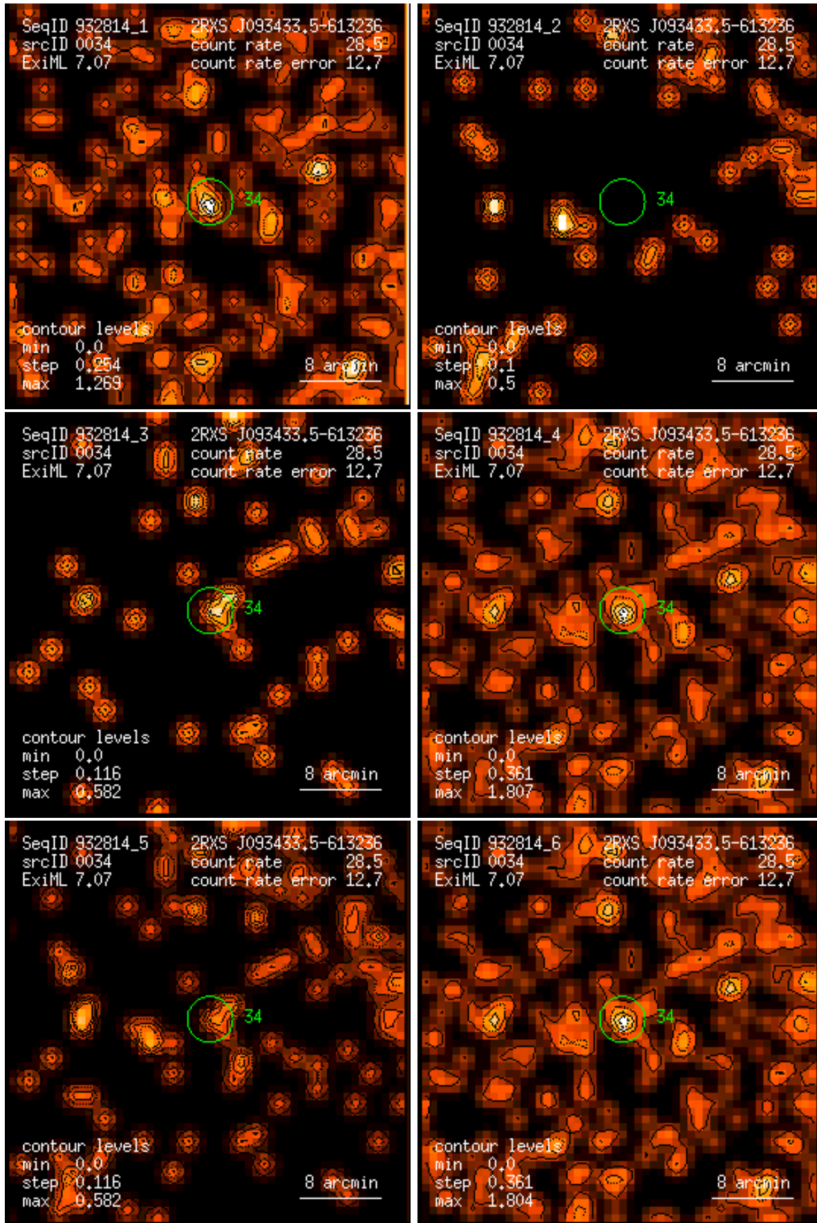
Figure 34: RASS 932814: detection 0034: band rate images, Gaussian filter: (1) PSPC channels 11 – 41, (2) 52 – 90, (3) 91 – 201, (4) 11 – 235, (5) 52 – 201, (6) 11 – 201. Broad band rates in counts/ks. Band rate contour levels in counts/ks/arcmin 2 .
