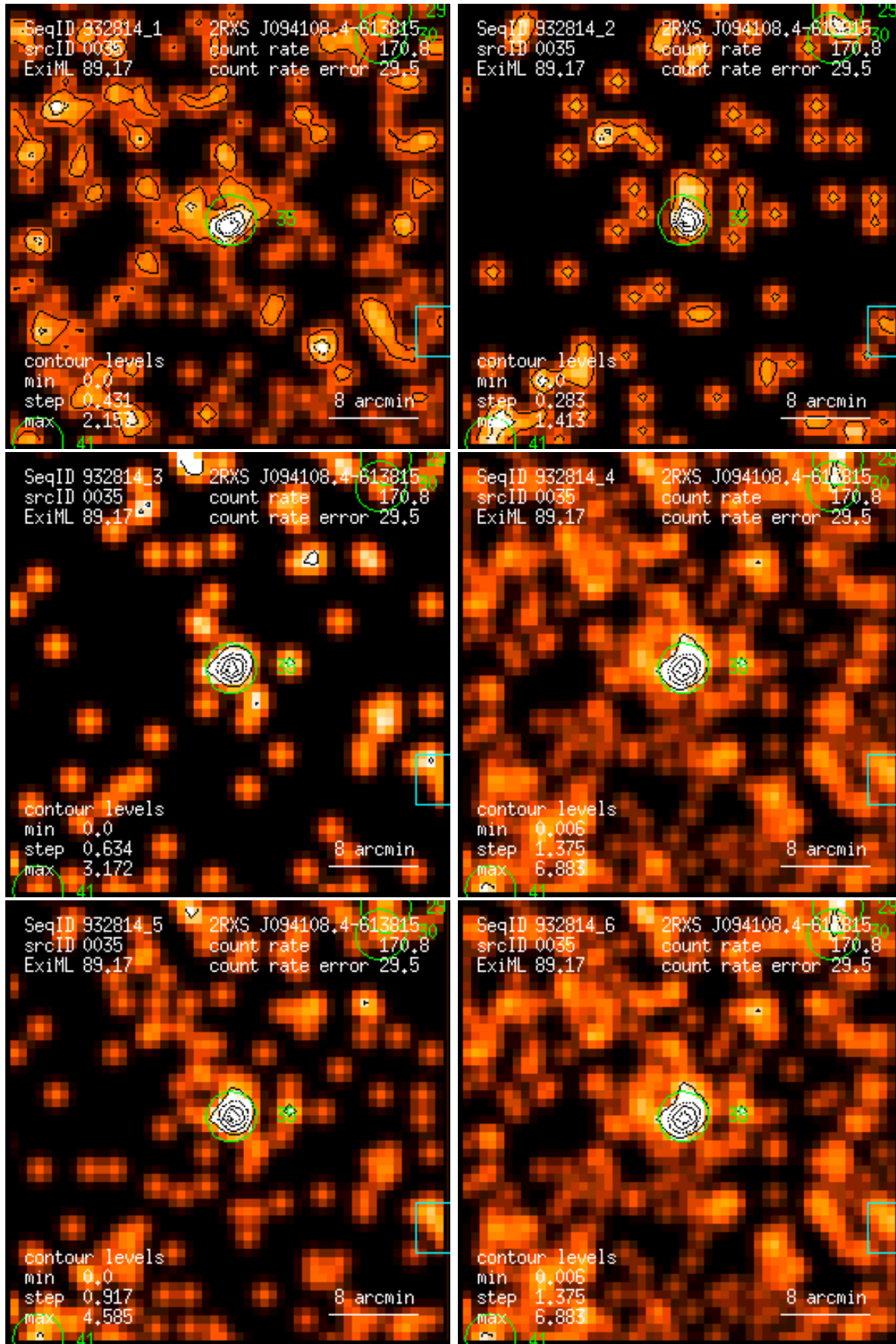
Figure 35: RASS 932814: detection 0035: band rate images, Gaussian filter: (1) PSPC channels 11 – 41, (2) 52 – 90, (3) 91 – 201, (4) 11 – 235, (5) 52 – 201, (6) 11 – 201. Broad band rates in counts/ks. Band rate contour levels in counts/ks/arcmin 2 .
