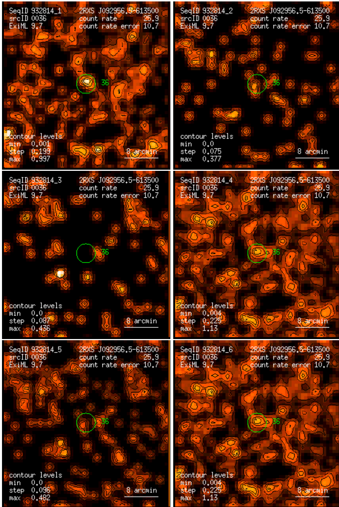
Figure 36: RASS 932814: detection 0036: band rate images, Gaussian filter: (1) PSPC channels 11 – 41, (2) 52 – 90, (3) 91 – 201, (4) 11 – 235, (5) 52 – 201, (6) 11 – 201. Broad band rates in counts/ks. Band rate contour levels in counts/ks/arcmin 2 .
