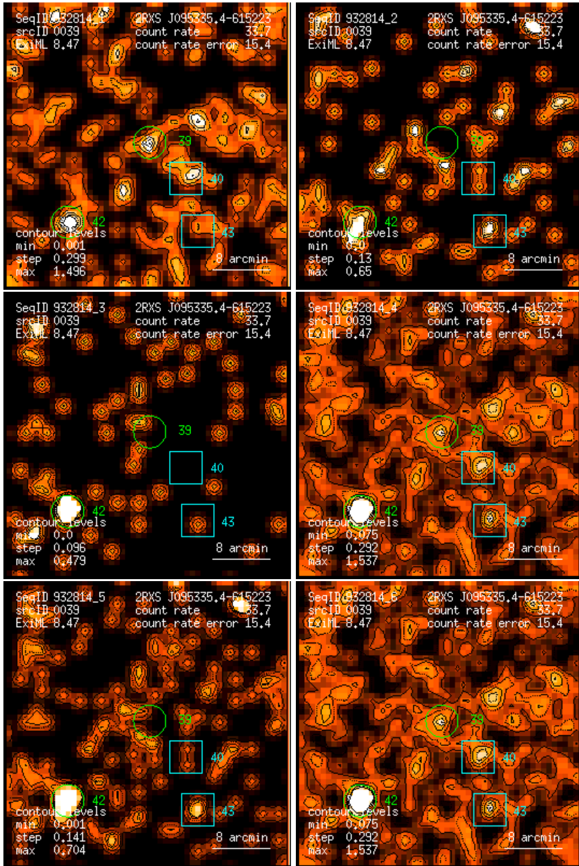
Figure 39: RASS 932814: detection 0039: band rate images, Gaussian filter: (1) PSPC channels 11 – 41, (2) 52 – 90, (3) 91 – 201, (4) 11 – 235, (5) 52 – 201, (6) 11 – 201. Broad band rates in counts/ks. Band rate contour levels in counts/ks/arcmin 2 .
