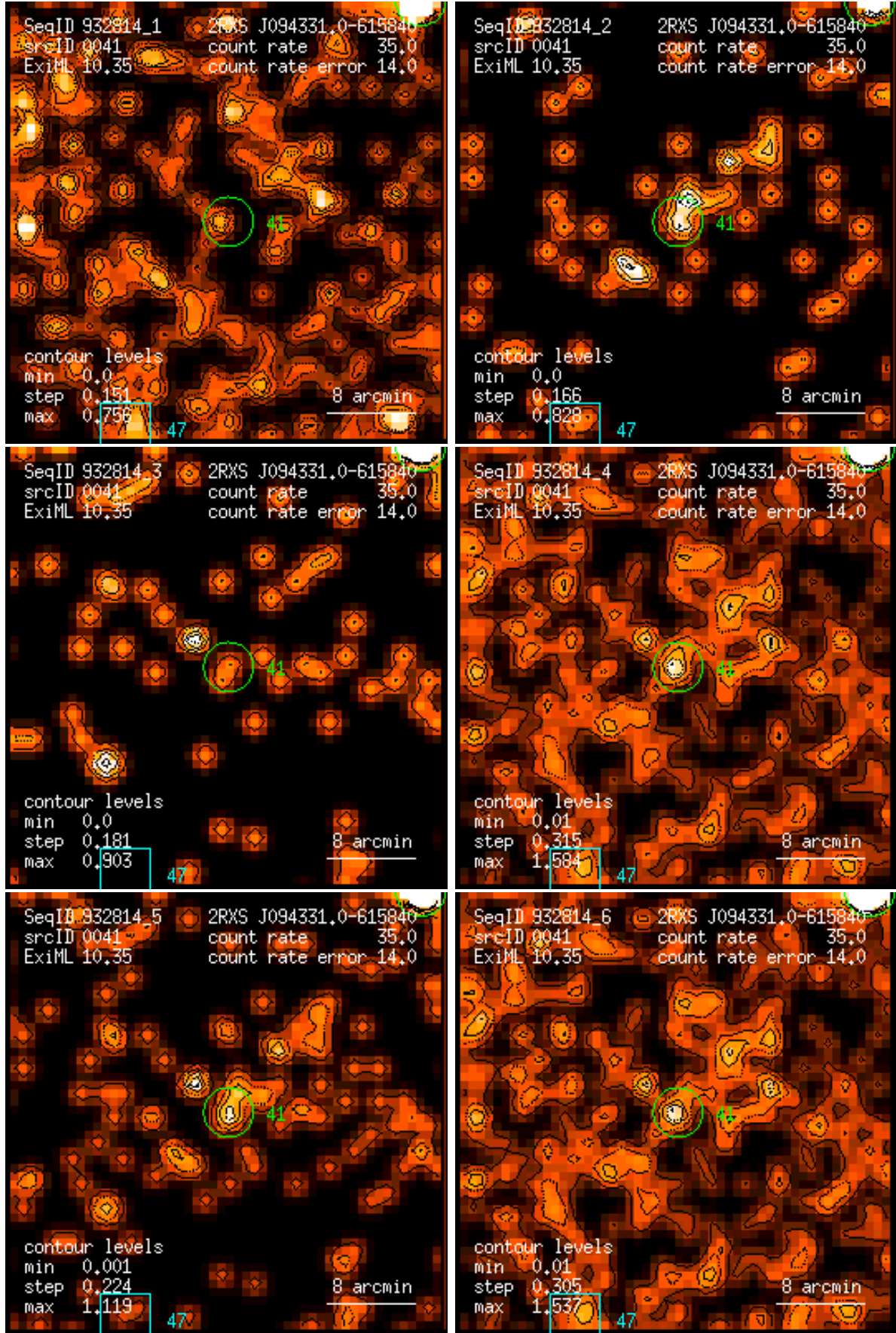
Figure 41: RASS 932814: detection 0041: band rate images, Gaussian filter: (1) PSPC channels 11 – 41, (2) 52 – 90, (3) 91 – 201, (4) 11 – 235, (5) 52 – 201, (6) 11 – 201. Broad band rates in counts/ks. Band rate contour levels in counts/ks/arcmin 2 .
