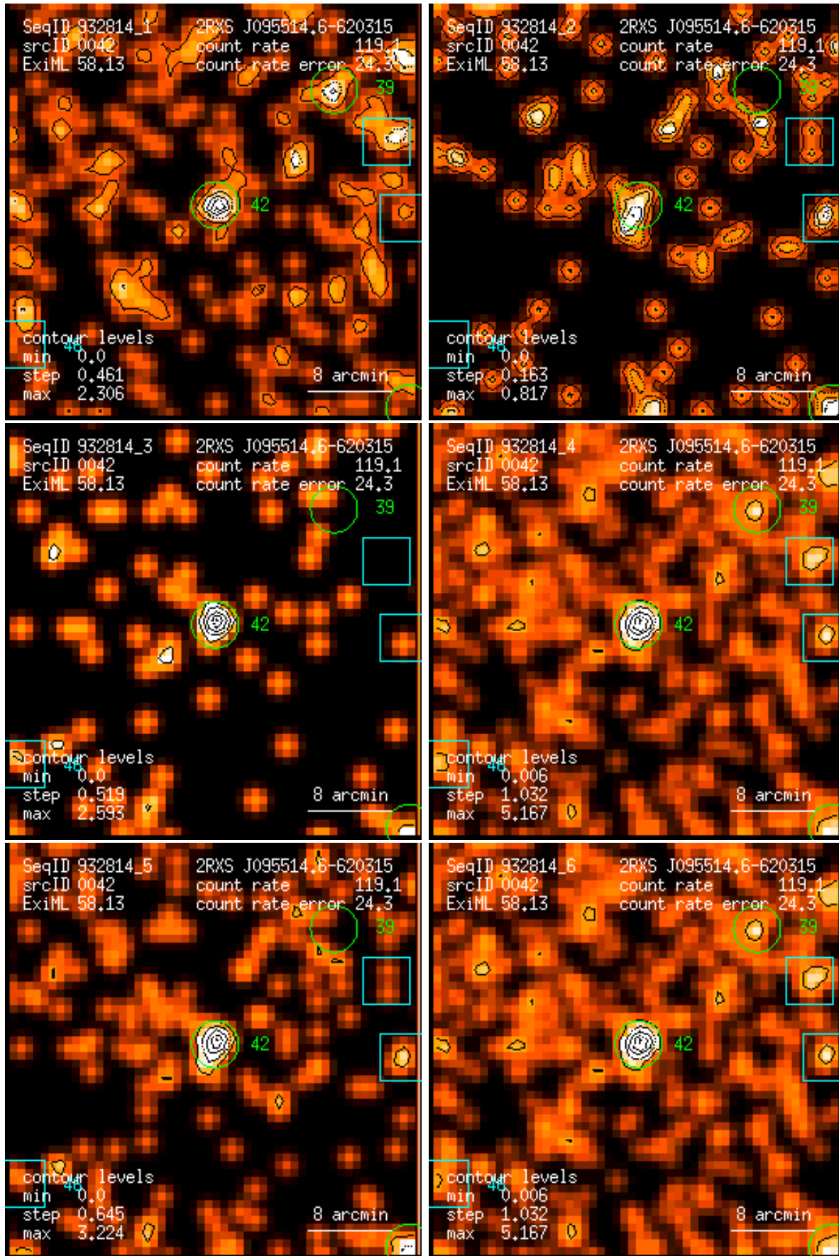
Figure 42: RASS 932814: detection 0042: band rate images, Gaussian filter: (1) PSPC channels 11 – 41, (2) 52 – 90, (3) 91 – 201, (4) 11 – 235, (5) 52 – 201, (6) 11 – 201. Broad band rates in counts/ks. Band rate contour levels in counts/ks/arcmin 2 .
