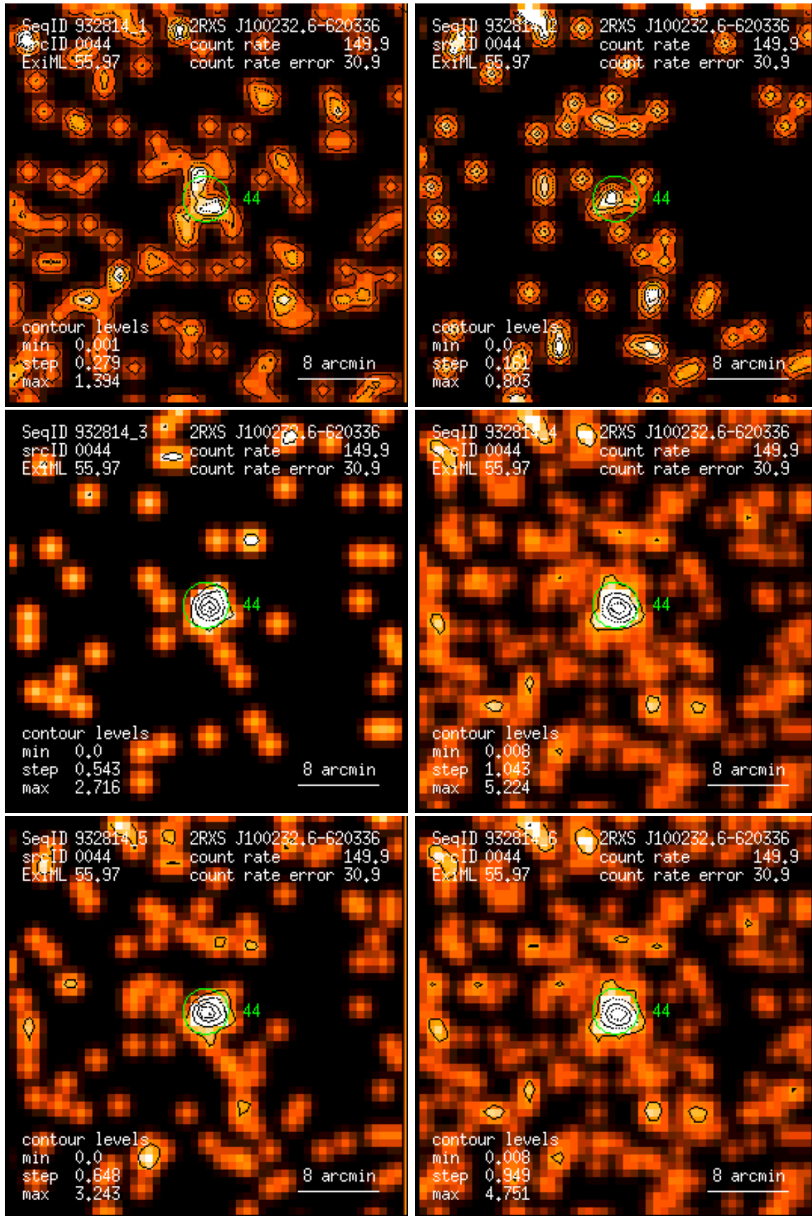
Figure 44: RASS 932814: detection 0044: band rate images, Gaussian filter: (1) PSPC channels 11 – 41, (2) 52 – 90, (3) 91 – 201, (4) 11 – 235, (5) 52 – 201, (6) 11 – 201. Broad band rates in counts/ks. Band rate contour levels in counts/ks/arcmin 2 .
