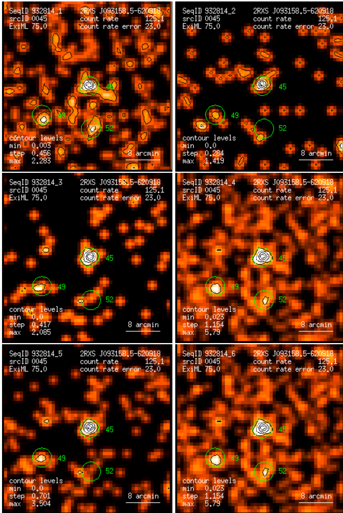
Figure 45: RASS 932814: detection 0045: band rate images, Gaussian filter: (1) PSPC channels 11 – 41, (2) 52 – 90, (3) 91 – 201, (4) 11 – 235, (5) 52 – 201, (6) 11 – 201. Broad band rates in counts/ks. Band rate contour levels in counts/ks/arcmin 2 .
