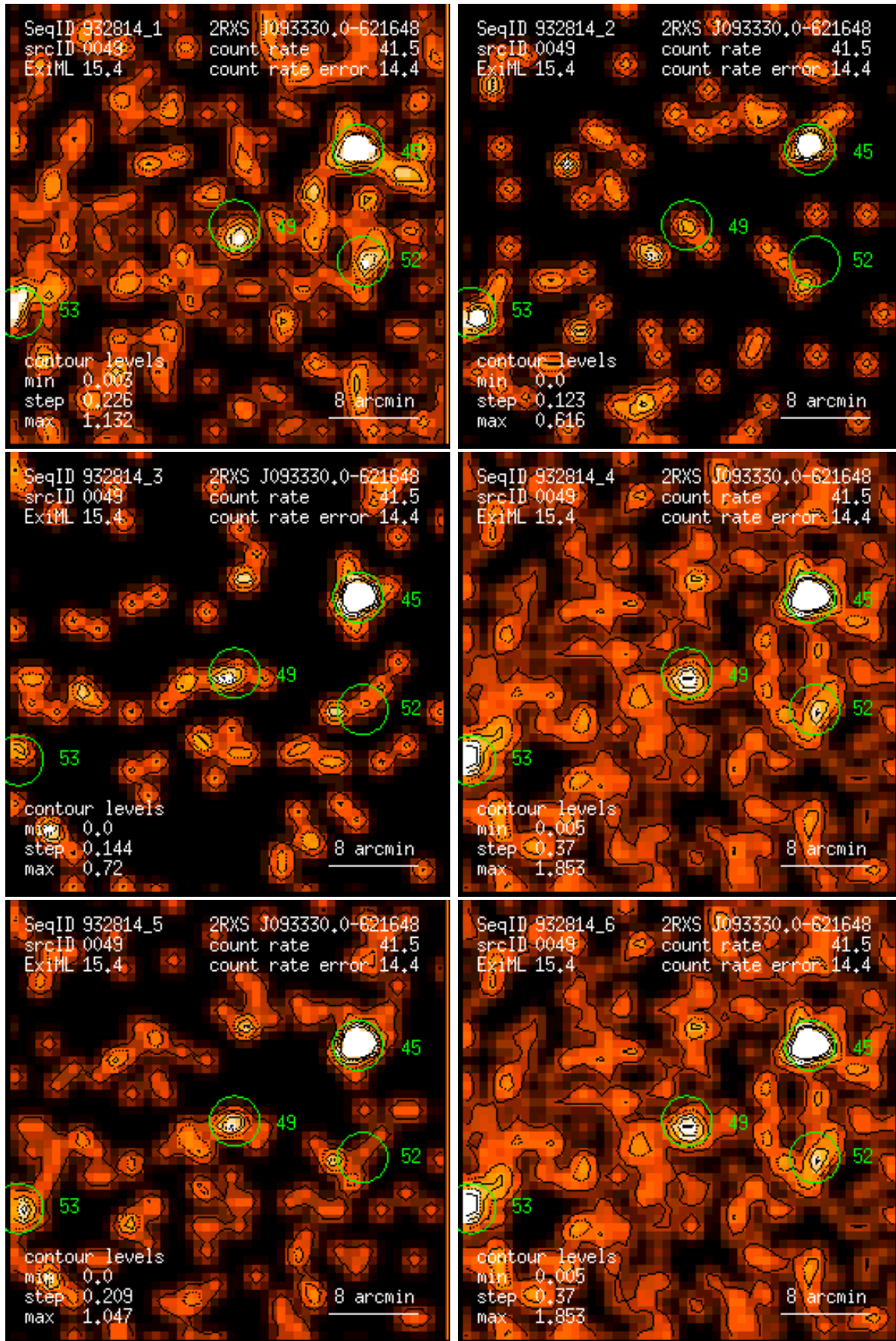
Figure 49: RASS 932814: detection 0049: band rate images, Gaussian filter: (1) PSPC channels 11 – 41, (2) 52 – 90, (3) 91 – 201, (4) 11 – 235, (5) 52 – 201, (6) 11 – 201. Broad band rates in counts/ks. Band rate contour levels in counts/ks/arcmin 2 .
