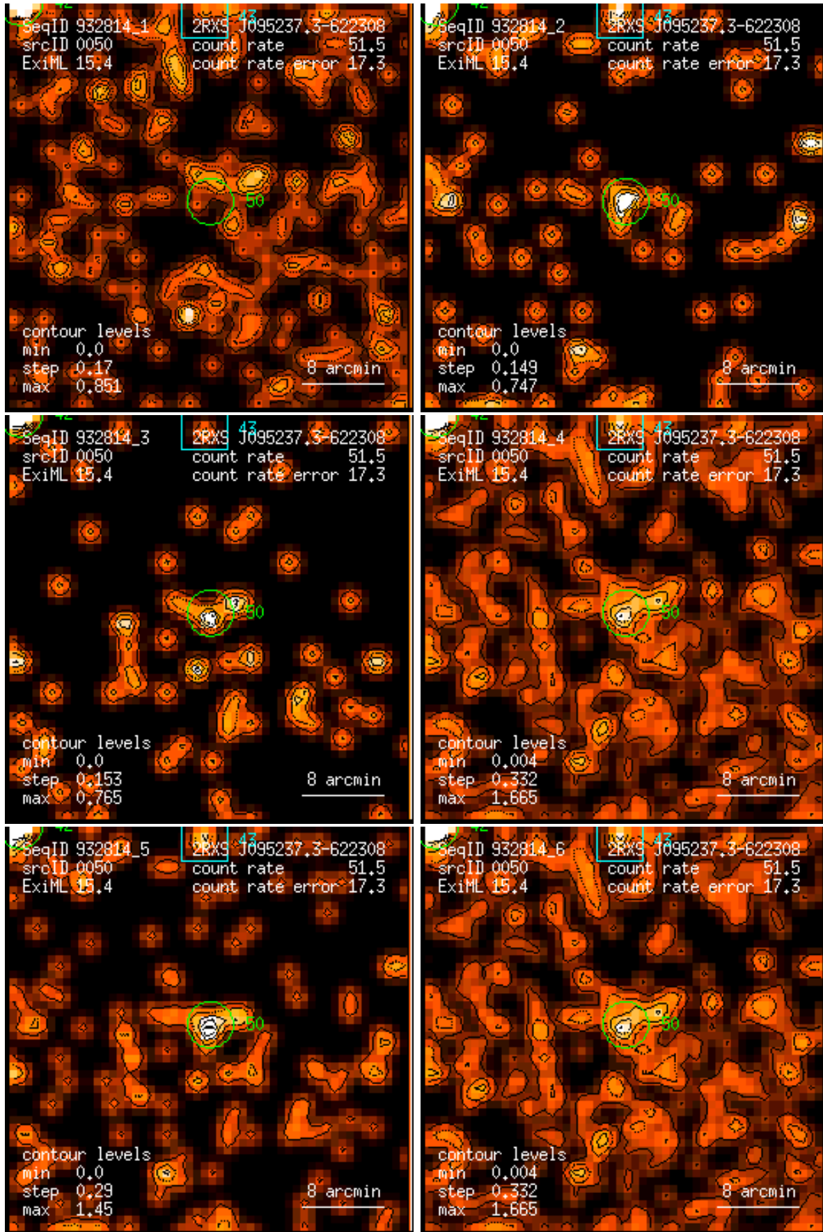
Figure 50: RASS 932814: detection 0050: band rate images, Gaussian filter: (1) PSPC channels 11 – 41, (2) 52 – 90, (3) 91 – 201, (4) 11 – 235, (5) 52 – 201, (6) 11 – 201. Broad band rates in counts/ks. Band rate contour levels in counts/ks/arcmin 2 .
