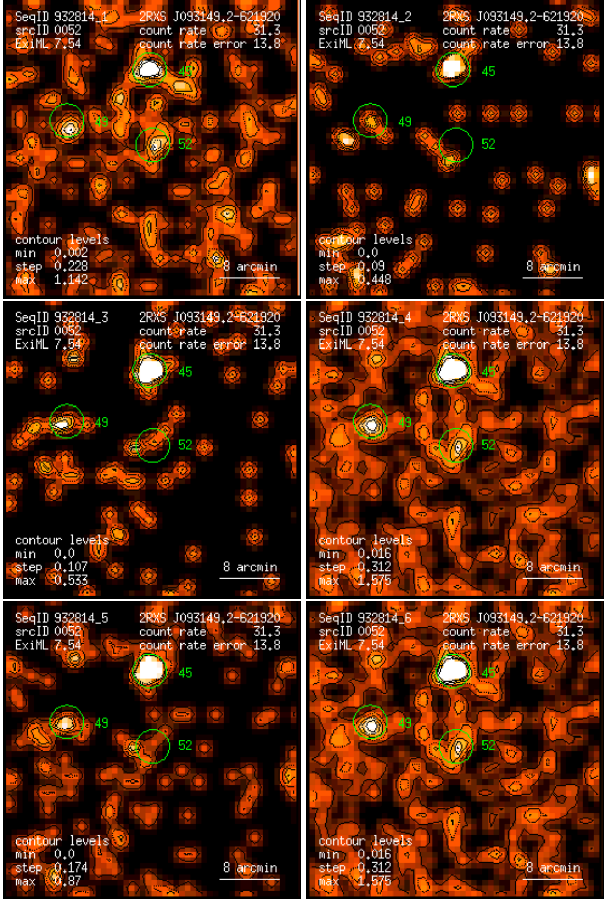
Figure 52: RASS 932814: detection 0052: band rate images, Gaussian filter: (1) PSPC channels 11 – 41, (2) 52 – 90, (3) 91 – 201, (4) 11 – 235, (5) 52 – 201, (6) 11 – 201. Broad band rates in counts/ks. Band rate contour levels in counts/ks/arcmin 2 .
