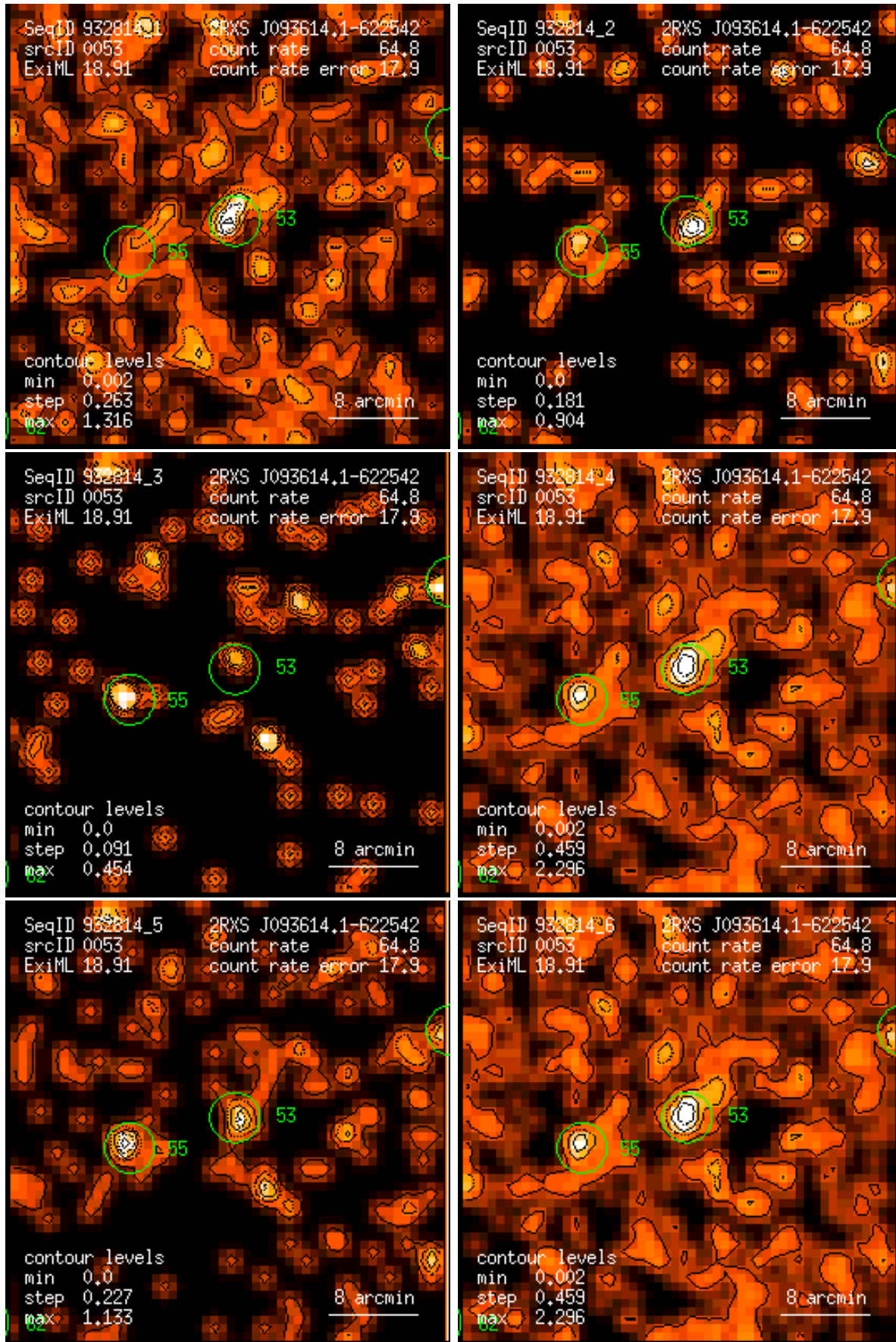
Figure 53: RASS 932814: detection 0053: band rate images, Gaussian filter: (1) PSPC channels 11 – 41, (2) 52 – 90, (3) 91 – 201, (4) 11 – 235, (5) 52 – 201, (6) 11 – 201. Broad band rates in counts/ks. Band rate contour levels in counts/ks/arcmin 2 .
