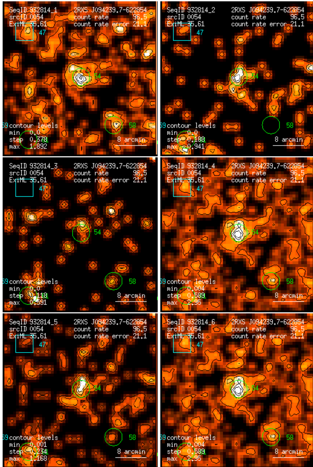
Figure 54: RASS 932814: detection 0054: band rate images, Gaussian filter: (1) PSPC channels 11 – 41, (2) 52 – 90, (3) 91 – 201, (4) 11 – 235, (5) 52 – 201, (6) 11 – 201. Broad band rates in counts/ks. Band rate contour levels in counts/ks/arcmin 2 .
