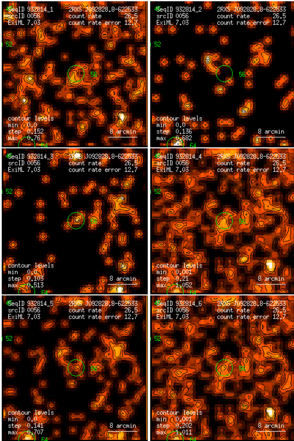
Figure 56: RASS 932814: detection 0056: band rate images, Gaussian filter: (1) PSPC channels 11 – 41, (2) 52 – 90, (3) 91 – 201, (4) 11 – 235, (5) 52 – 201, (6) 11 – 201. Broad band rates in counts/ks. Band rate contour levels in counts/ks/arcmin 2 .
