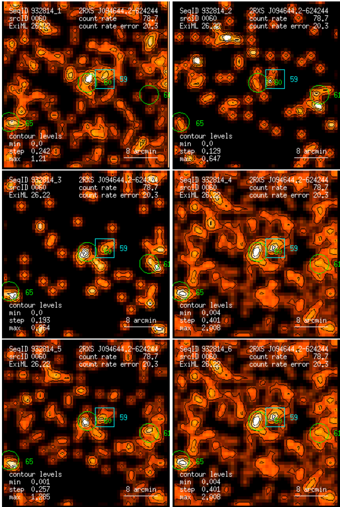
Figure 60: RASS 932814: detection 0060: band rate images, Gaussian filter: (1) PSPC channels 11 – 41, (2) 52 – 90, (3) 91 – 201, (4) 11 – 235, (5) 52 – 201, (6) 11 – 201. Broad band rates in counts/ks. Band rate contour levels in counts/ks/arcmin 2 .
