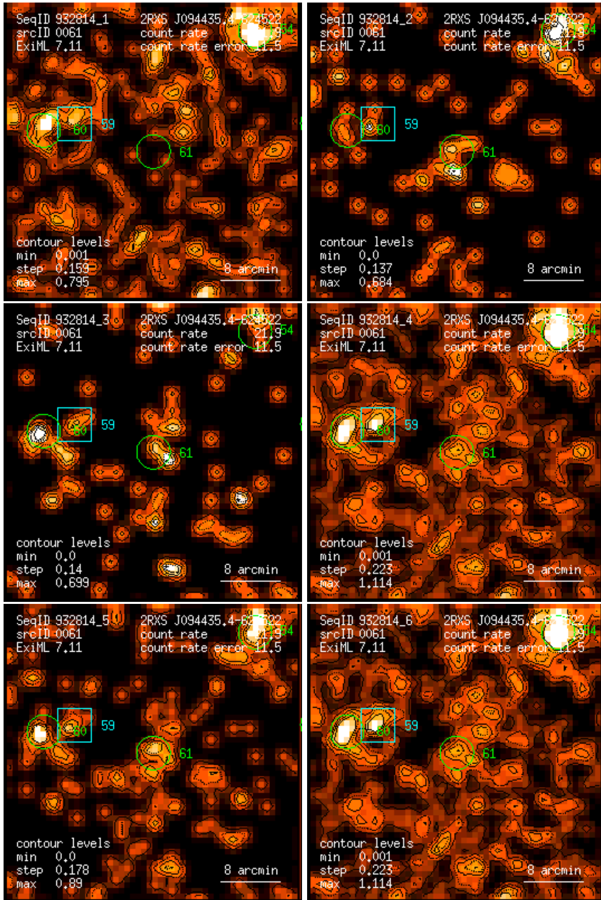
Figure 61: RASS 932814: detection 0061: band rate images, Gaussian filter: (1) PSPC channels 11 – 41, (2) 52 – 90, (3) 91 – 201, (4) 11 – 235, (5) 52 – 201, (6) 11 – 201. Broad band rates in counts/ks. Band rate contour levels in counts/ks/arcmin 2 .
