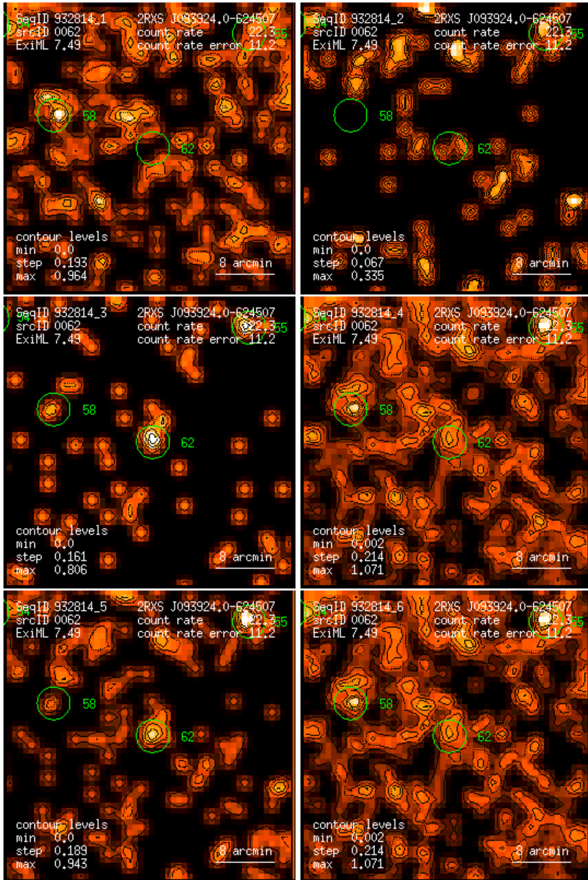
Figure 62: RASS 932814: detection 0062: band rate images, Gaussian filter: (1) PSPC channels 11 – 41, (2) 52 – 90, (3) 91 – 201, (4) 11 – 235, (5) 52 – 201, (6) 11 – 201. Broad band rates in counts/ks. Band rate contour levels in counts/ks/arcmin 2 .
