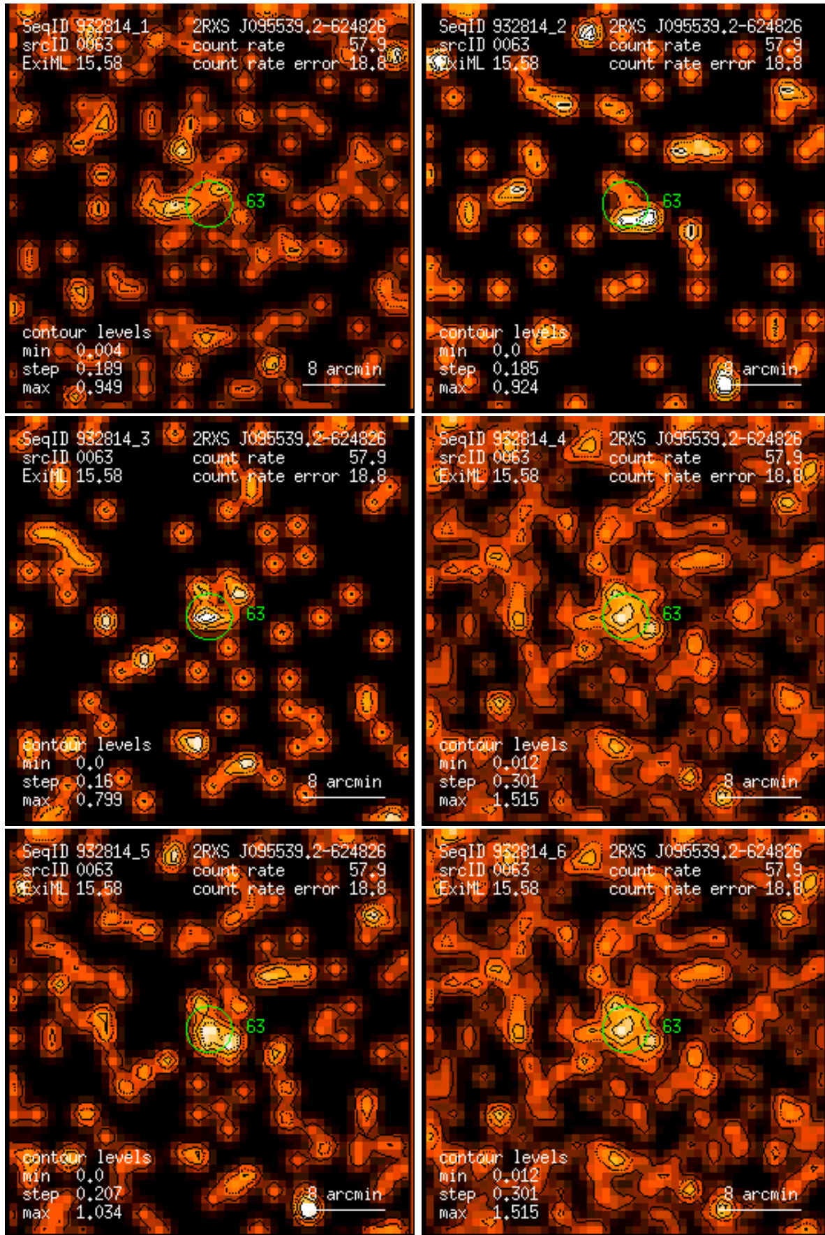
Figure 63: RASS 932814: detection 0063: band rate images, Gaussian filter: (1) PSPC channels 11 – 41, (2) 52 – 90, (3) 91 – 201, (4) 11 – 235, (5) 52 – 201, (6) 11 – 201. Broad band rates in counts/ks. Band rate contour levels in counts/ks/arcmin 2 .
