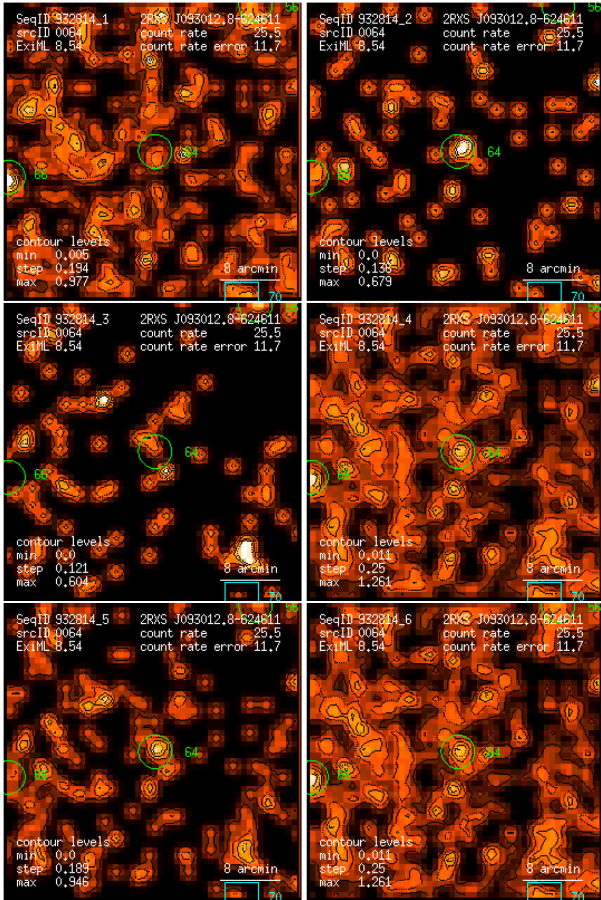
Figure 64: RASS 932814: detection 0064: band rate images, Gaussian filter: (1) PSPC channels 11 – 41, (2) 52 – 90, (3) 91 – 201, (4) 11 – 235, (5) 52 – 201, (6) 11 – 201. Broad band rates in counts/ks. Band rate contour levels in counts/ks/arcmin 2 .
