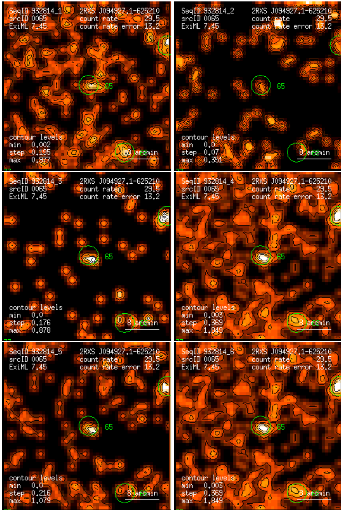
Figure 65: RASS 932814: detection 0065: band rate images, Gaussian filter: (1) PSPC channels 11 – 41, (2) 52 – 90, (3) 91 – 201, (4) 11 – 235, (5) 52 – 201, (6) 11 – 201. Broad band rates in counts/ks. Band rate contour levels in counts/ks/arcmin 2 .
