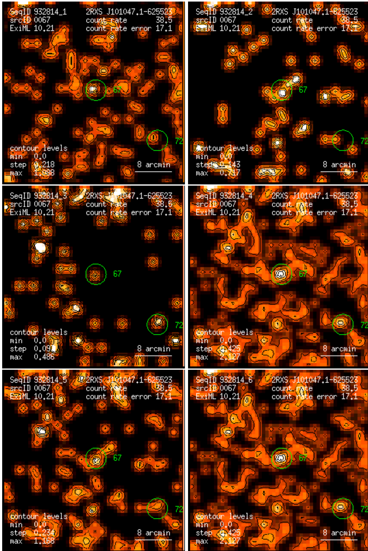
Figure 67: RASS 932814: detection 0067: band rate images, Gaussian filter: (1) PSPC channels 11 – 41, (2) 52 – 90, (3) 91 – 201, (4) 11 – 235, (5) 52 – 201, (6) 11 – 201. Broad band rates in counts/ks. Band rate contour levels in counts/ks/arcmin 2 .
