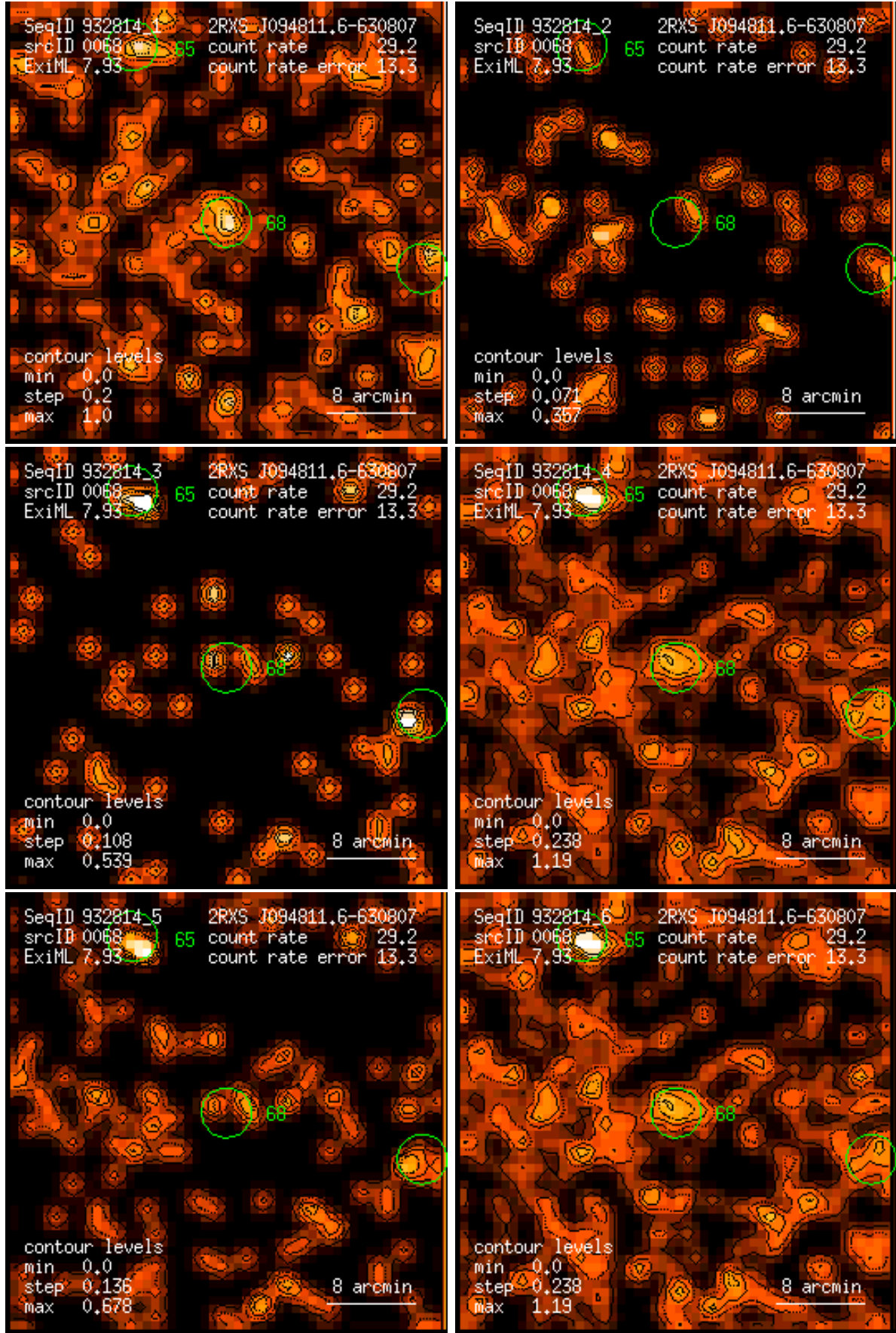
Figure 68: RASS 932814: detection 0068: band rate images, Gaussian filter: (1) PSPC channels 11 – 41, (2) 52 – 90, (3) 91 – 201, (4) 11 – 235, (5) 52 – 201, (6) 11 – 201. Broad band rates in counts/ks. Band rate contour levels in counts/ks/arcmin 2 .
