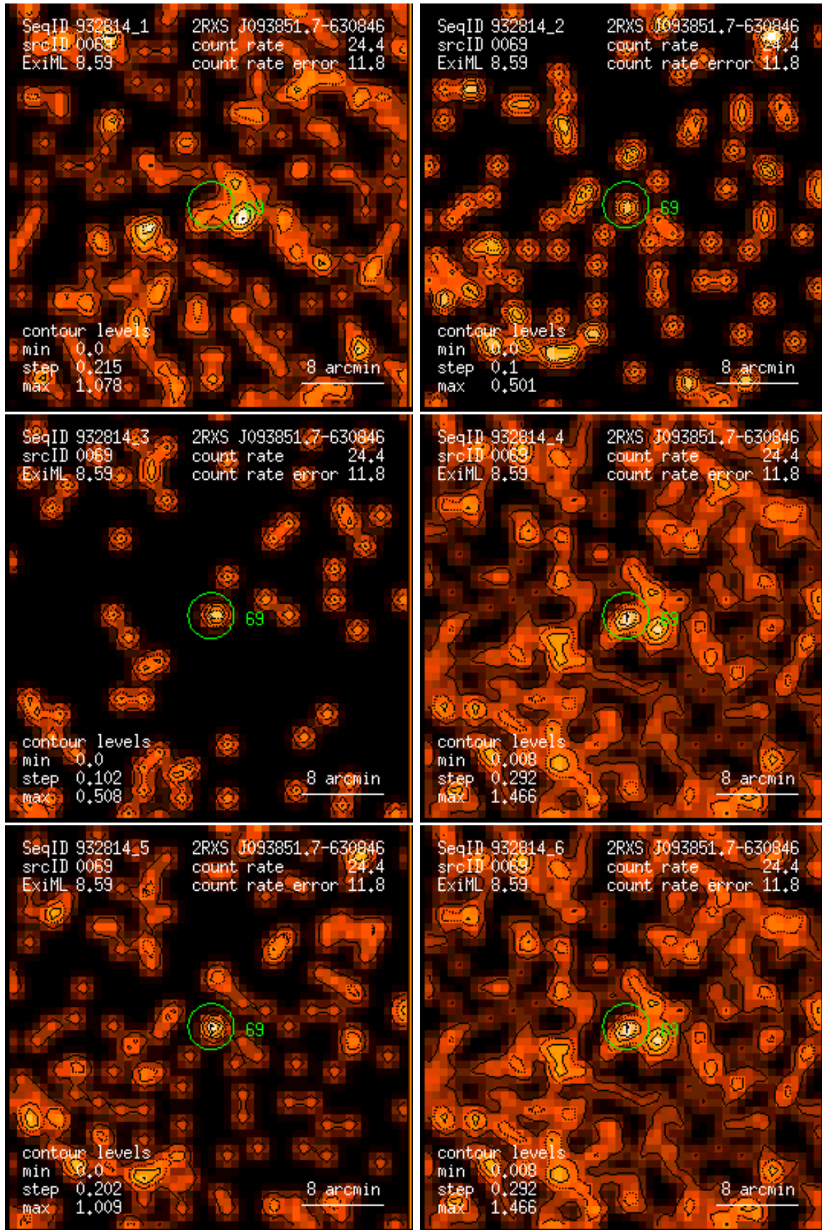
Figure 69: RASS 932814: detection 0069: band rate images, Gaussian filter: (1) PSPC channels 11 – 41, (2) 52 – 90, (3) 91 – 201, (4) 11 – 235, (5) 52 – 201, (6) 11 – 201. Broad band rates in counts/ks. Band rate contour levels in counts/ks/arcmin 2 .
