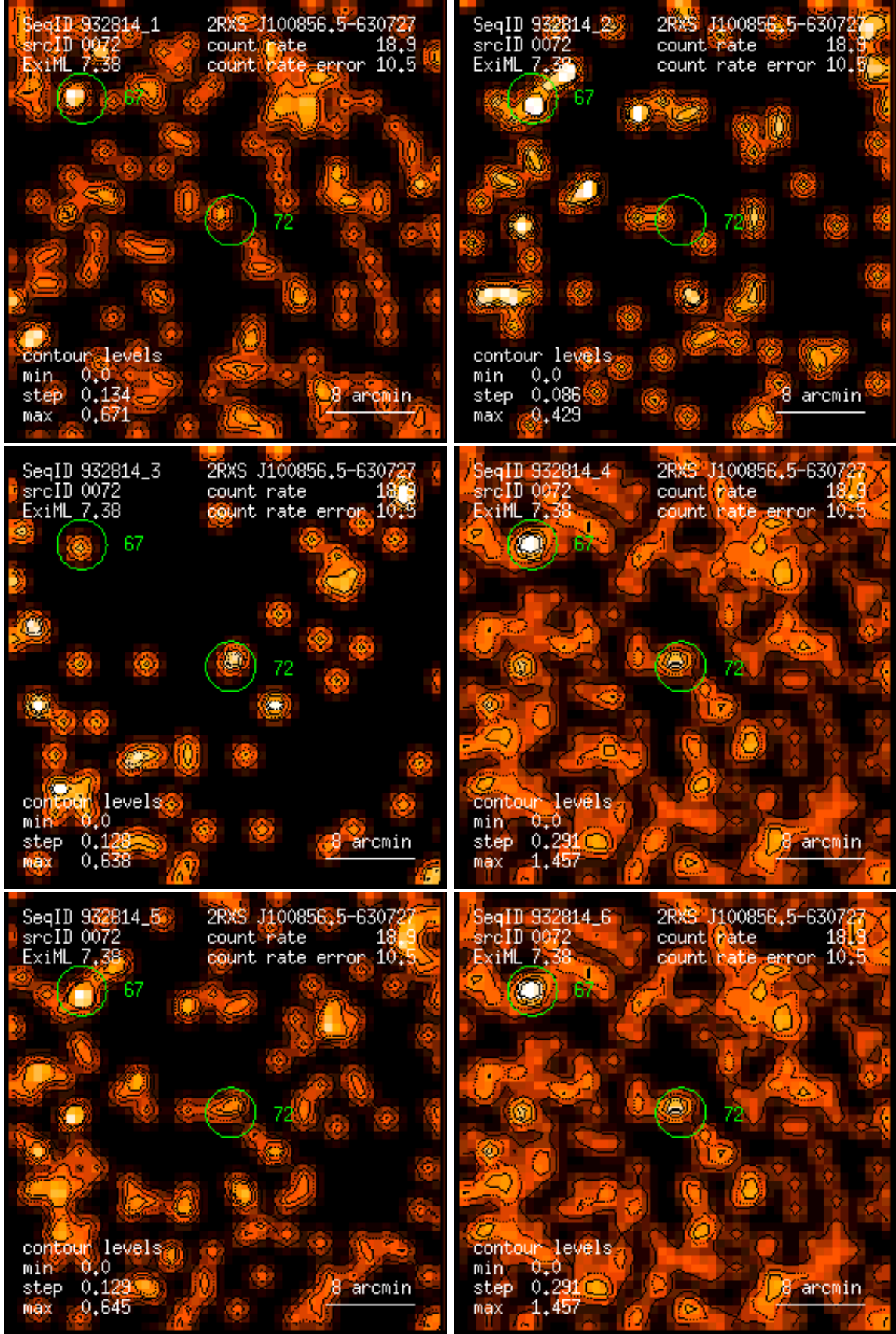
Figure 72: RASS 932814: detection 0072: band rate images, Gaussian filter: (1) PSPC channels 11 – 41, (2) 52 – 90, (3) 91 – 201, (4) 11 – 235, (5) 52 – 201, (6) 11 – 201. Broad band rates in counts/ks. Band rate contour levels in counts/ks/arcmin 2 .
