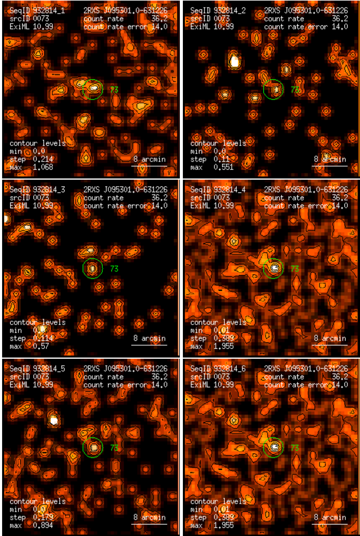
Figure 73: RASS 932814: detection 0073: band rate images, Gaussian filter: (1) PSPC channels 11 – 41, (2) 52 – 90, (3) 91 – 201, (4) 11 – 235, (5) 52 – 201, (6) 11 – 201. Broad band rates in counts/ks. Band rate contour levels in counts/ks/arcmin 2 .
