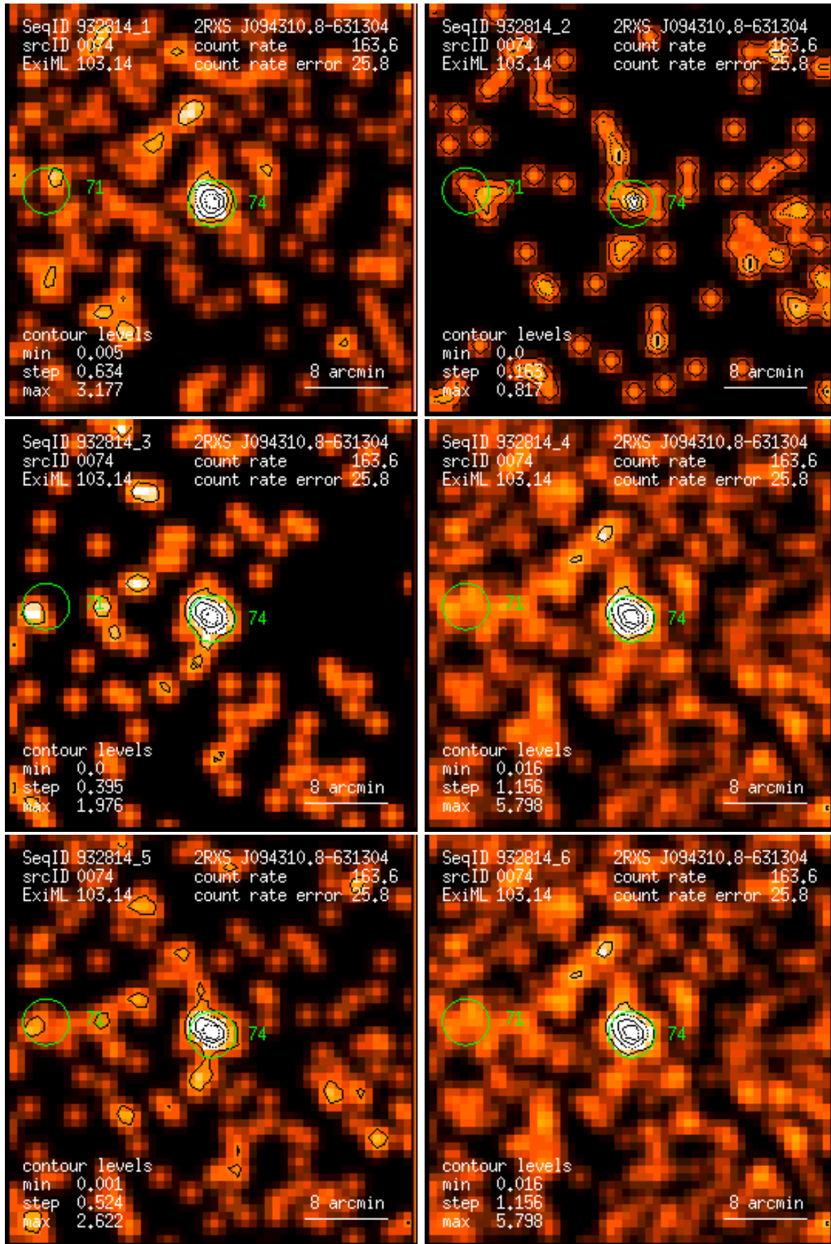
Figure 74: RASS 932814: detection 0074: band rate images, Gaussian filter: (1) PSPC channels 11 – 41, (2) 52 – 90, (3) 91 – 201, (4) 11 – 235, (5) 52 – 201, (6) 11 – 201. Broad band rates in counts/ks. Band rate contour levels in counts/ks/arcmin 2 .
