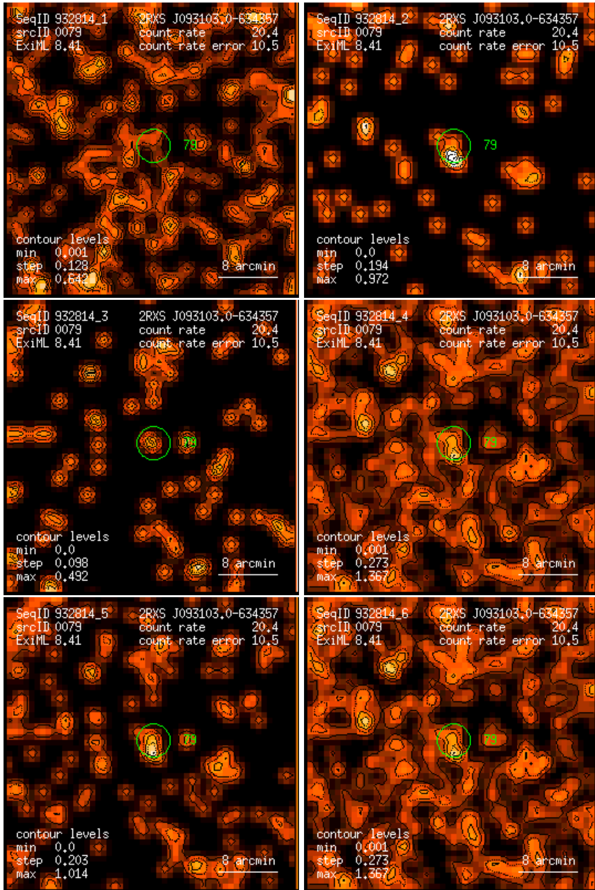
Figure 79: RASS 932814: detection 0079: band rate images, Gaussian filter: (1) PSPC channels 11 – 41, (2) 52 – 90, (3) 91 – 201, (4) 11 – 235, (5) 52 – 201, (6) 11 – 201. Broad band rates in counts/ks. Band rate contour levels in counts/ks/arcmin 2 .
