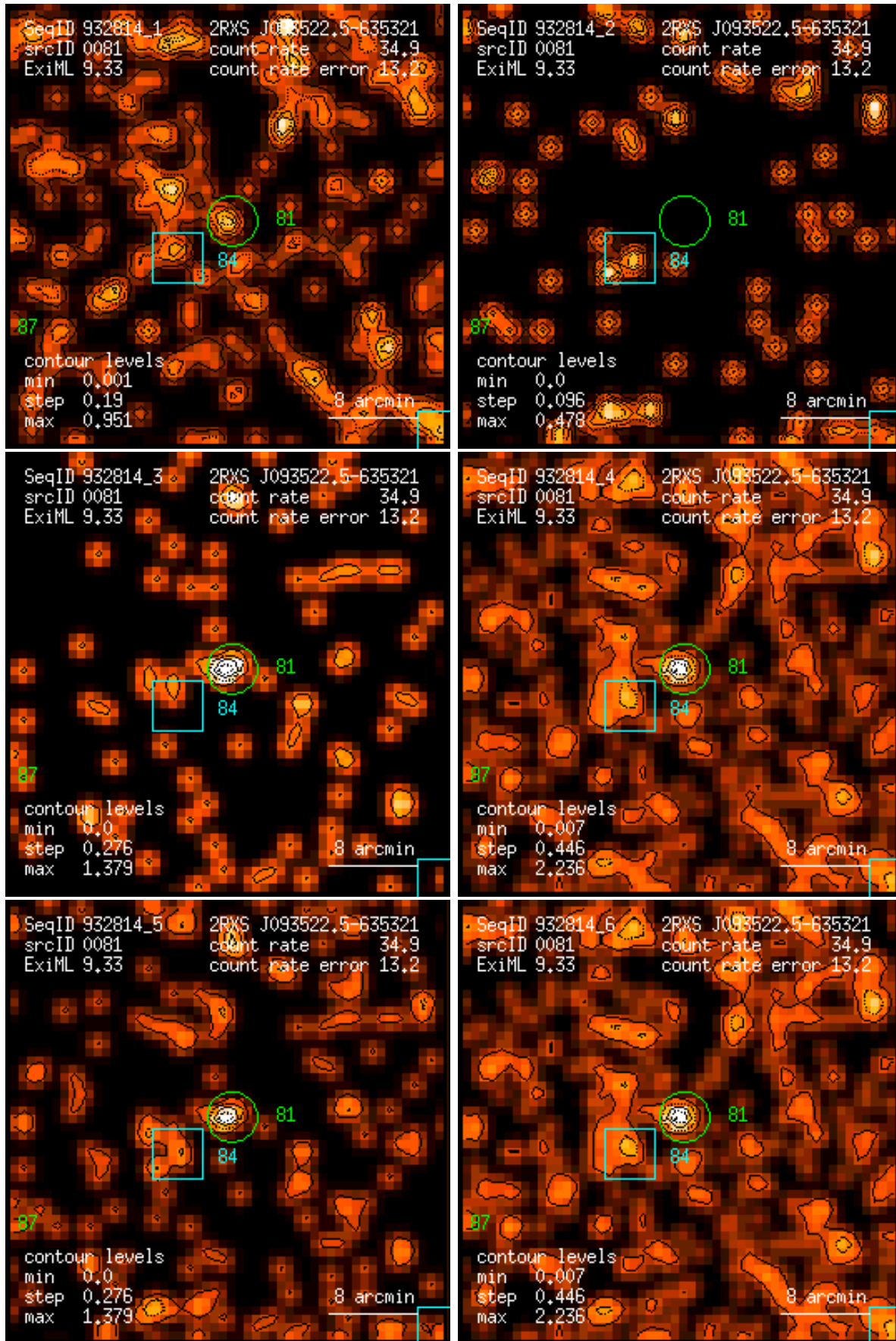
Figure 81: RASS 932814: detection 0081: band rate images, Gaussian filter: (1) PSPC channels 11 – 41, (2) 52 – 90, (3) 91 – 201, (4) 11 – 235, (5) 52 – 201, (6) 11 – 201. Broad band rates in counts/ks. Band rate contour levels in counts/ks/arcmin 2 .
