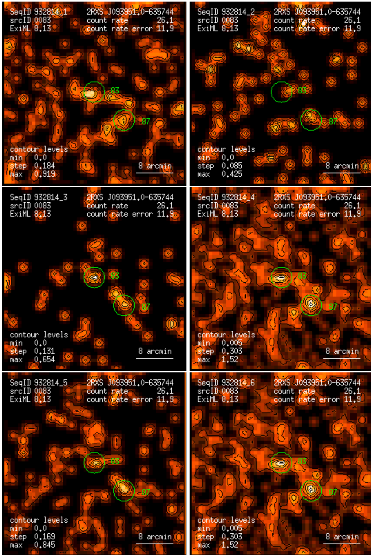
Figure 83: RASS 932814: detection 0083: band rate images, Gaussian filter: (1) PSPC channels 11 – 41, (2) 52 – 90, (3) 91 – 201, (4) 11 – 235, (5) 52 – 201, (6) 11 – 201. Broad band rates in counts/ks. Band rate contour levels in counts/ks/arcmin 2 .
