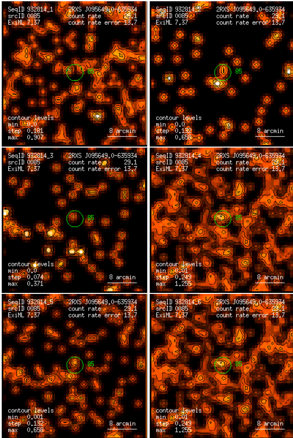
Figure 85: RASS 932814: detection 0085: band rate images, Gaussian filter: (1) PSPC channels 11 – 41, (2) 52 – 90, (3) 91 – 201, (4) 11 – 235, (5) 52 – 201, (6) 11 – 201. Broad band rates in counts/ks. Band rate contour levels in counts/ks/arcmin 2 .
