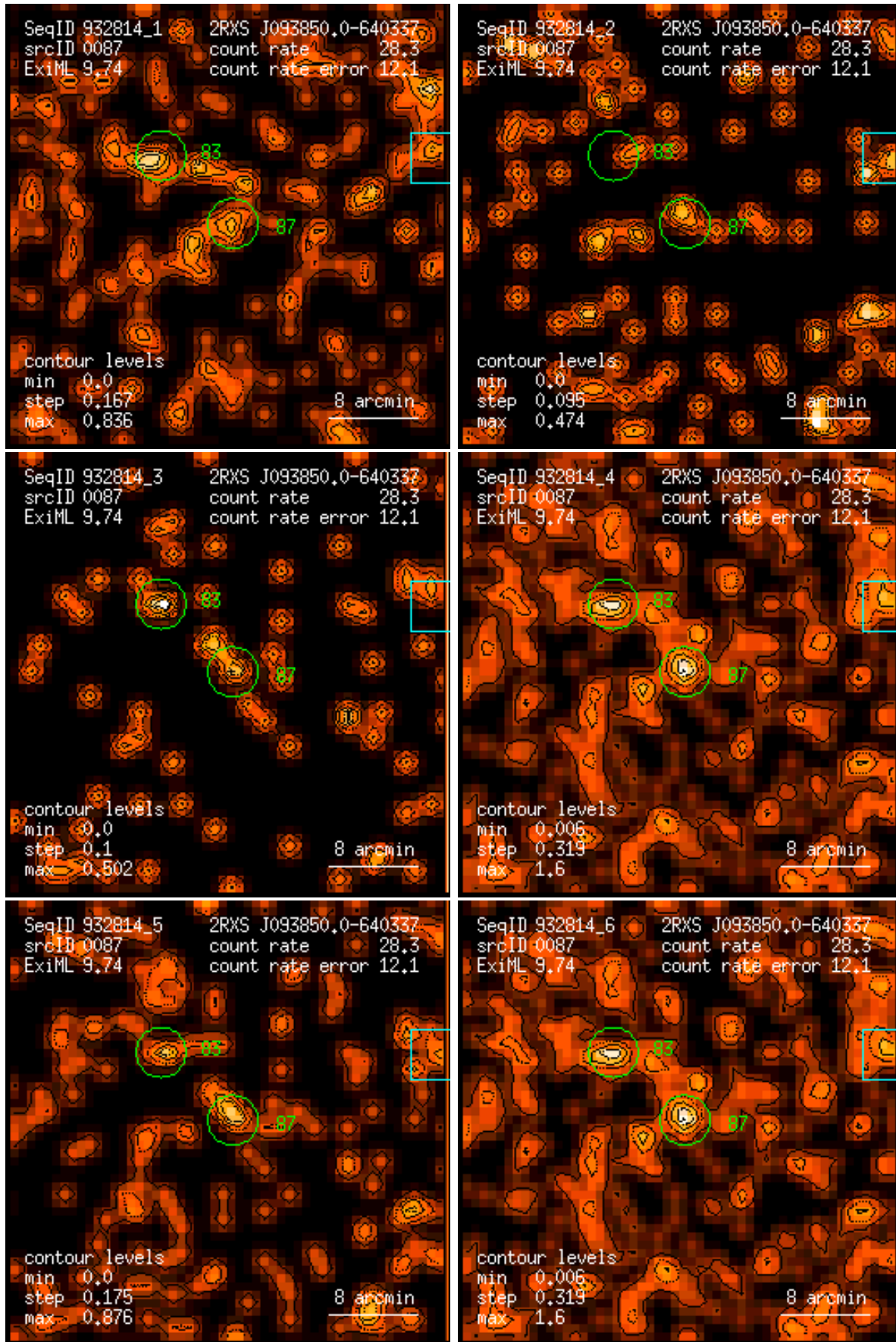
Figure 87: RASS 932814: detection 0087: band rate images, Gaussian filter: (1) PSPC channels 11 – 41, (2) 52 – 90, (3) 91 – 201, (4) 11 – 235, (5) 52 – 201, (6) 11 – 201. Broad band rates in counts/ks. Band rate contour levels in counts/ks/arcmin 2 .
