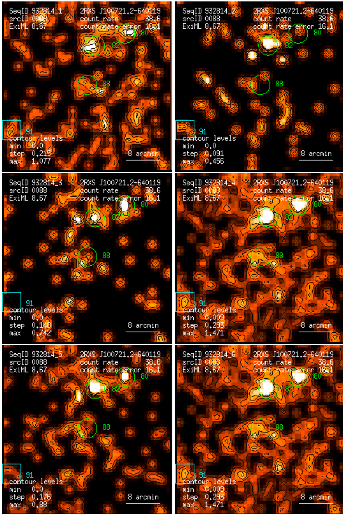
Figure 88: RASS 932814: detection 0088: band rate images, Gaussian filter: (1) PSPC channels 11 – 41, (2) 52 – 90, (3) 91 – 201, (4) 11 – 235, (5) 52 – 201, (6) 11 – 201. Broad band rates in counts/ks. Band rate contour levels in counts/ks/arcmin 2 .
