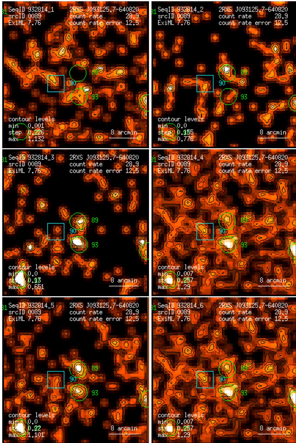
Figure 89: RASS 932814: detection 0089: band rate images, Gaussian filter: (1) PSPC channels 11 – 41, (2) 52 – 90, (3) 91 – 201, (4) 11 – 235, (5) 52 – 201, (6) 11 – 201. Broad band rates in counts/ks. Band rate contour levels in counts/ks/arcmin 2 .
