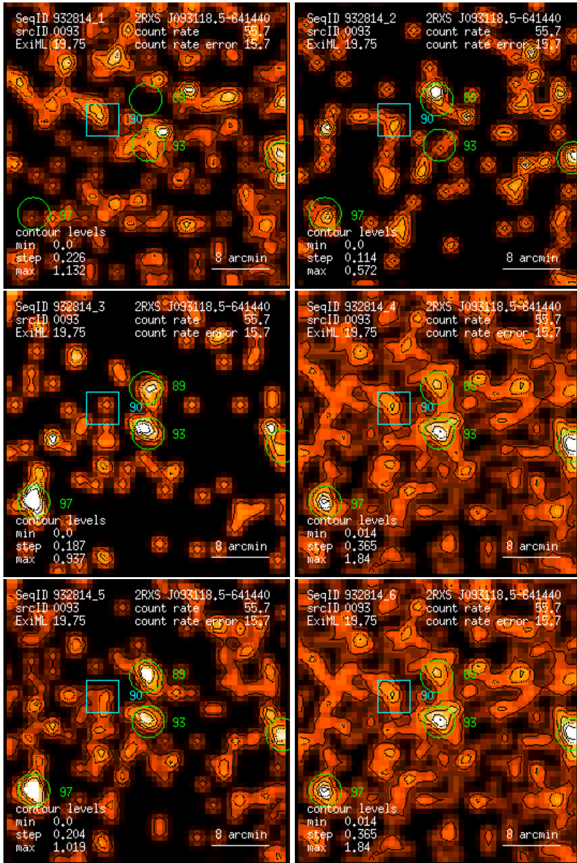
Figure 93: RASS 932814: detection 0093: band rate images, Gaussian filter: (1) PSPC channels 11 – 41, (2) 52 – 90, (3) 91 – 201, (4) 11 – 235, (5) 52 – 201, (6) 11 – 201. Broad band rates in counts/ks. Band rate contour levels in counts/ks/arcmin 2 .
