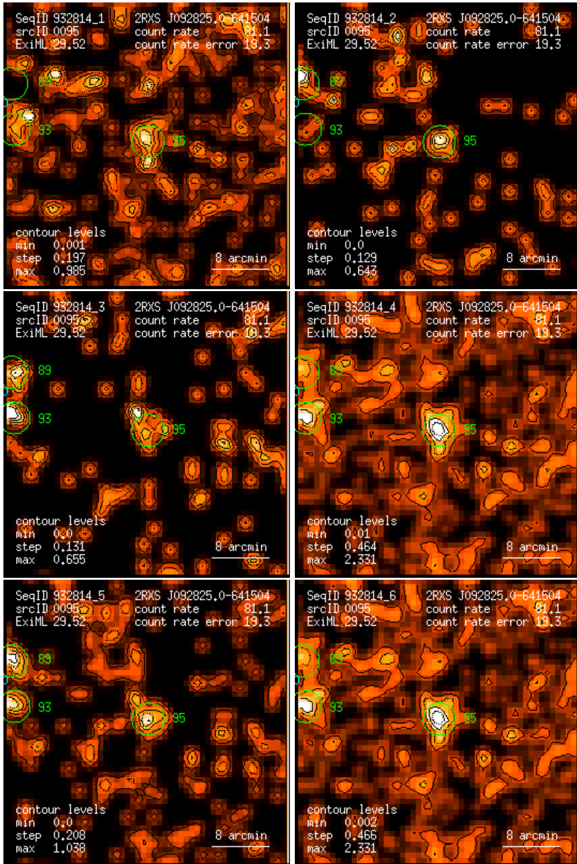
Figure 95: RASS 932814: detection 0095: band rate images, Gaussian filter: (1) PSPC channels 11 – 41, (2) 52 – 90, (3) 91 – 201, (4) 11 – 235, (5) 52 – 201, (6) 11 – 201. Broad band rates in counts/ks. Band rate contour levels in counts/ks/arcmin 2 .
