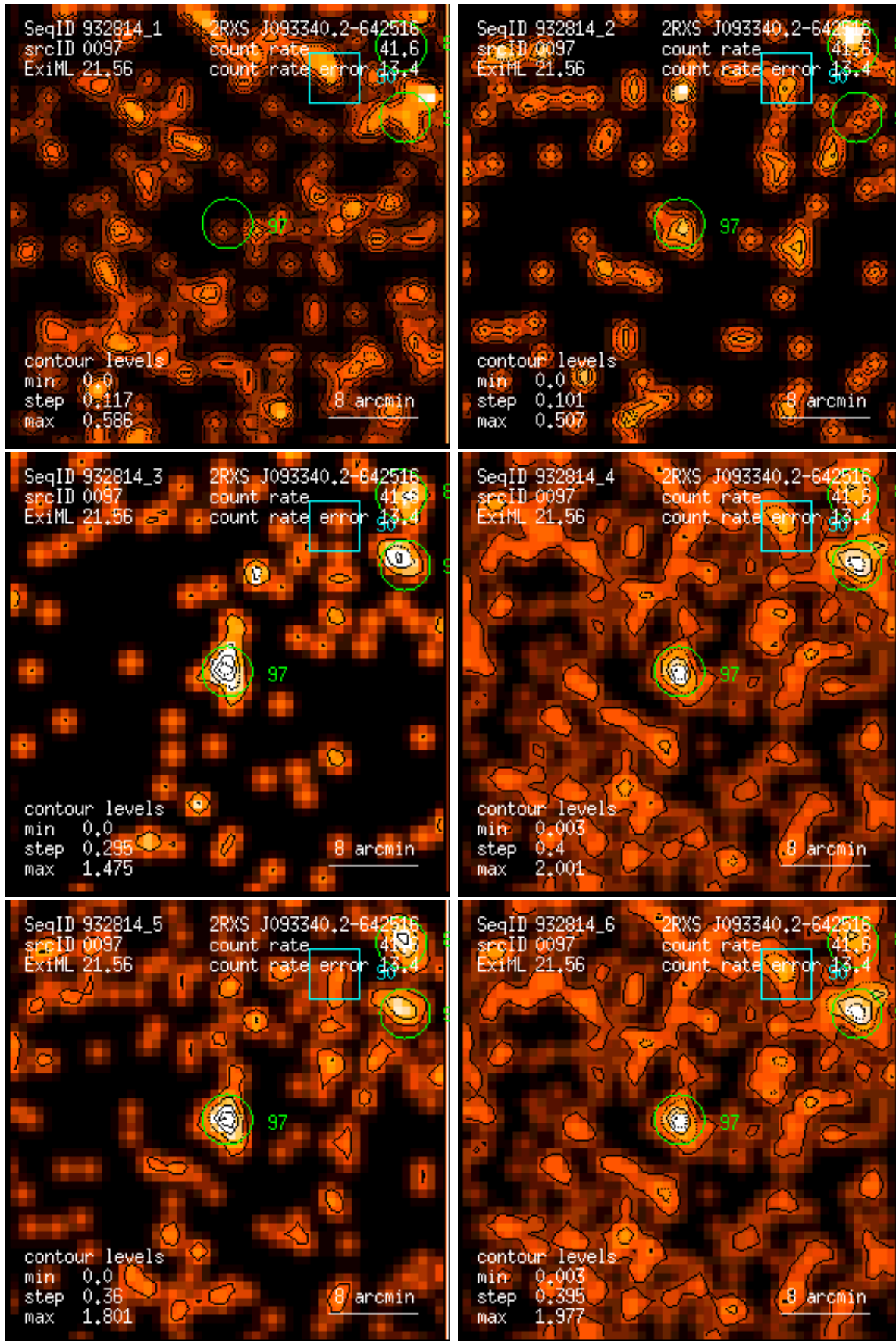
Figure 97: RASS 932814: detection 0097: band rate images, Gaussian filter: (1) PSPC channels 11 – 41, (2) 52 – 90, (3) 91 – 201, (4) 11 – 235, (5) 52 – 201, (6) 11 – 201. Broad band rates in counts/ks. Band rate contour levels in counts/ks/arcmin 2 .
