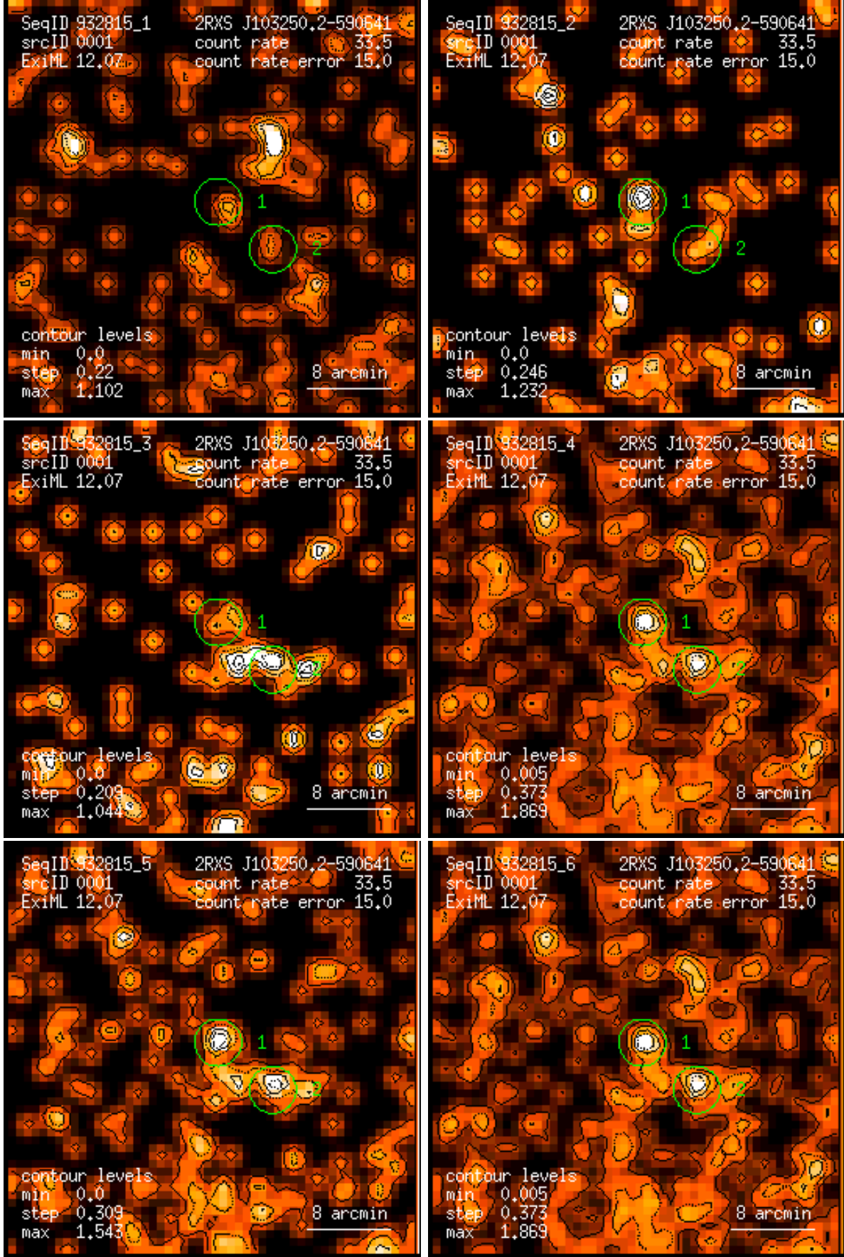
Figure 1: RASS 932815: detection 0001: band rate images, Gaussian filter: (1) PSPC channels 11 – 41, (2) 52 – 90, (3) 91 – 201, (4) 11 – 235, (5) 52 – 201, (6) 11 – 201. Broad band rates in counts/ks. Band rate contour levels in counts/ks/arcmin 2 .
