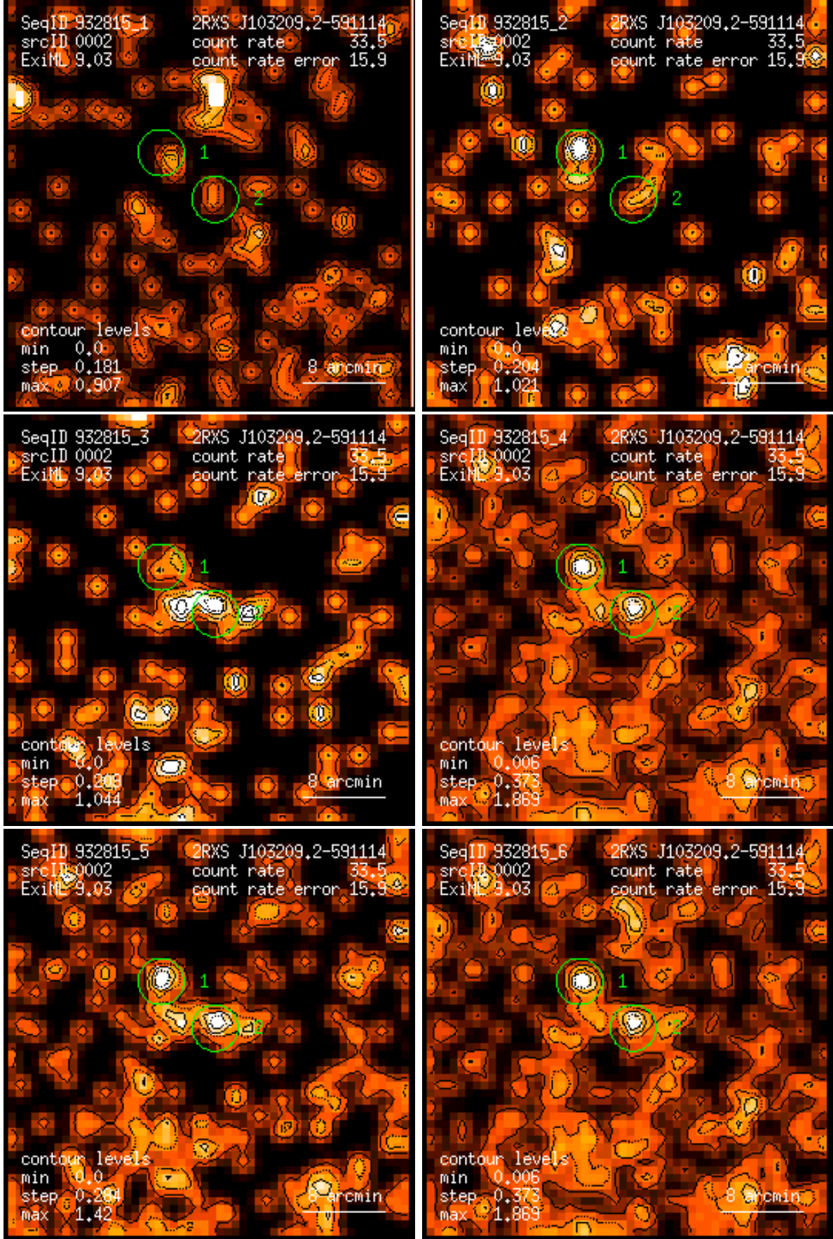
Figure 2: RASS 932815: detection 0002: band rate images, Gaussian filter: (1) PSPC channels 11 – 41, (2) 52 – 90, (3) 91 – 201, (4) 11 – 235, (5) 52 – 201, (6) 11 – 201. Broad band rates in counts/ks. Band rate contour levels in counts/ks/arcmin 2 .
