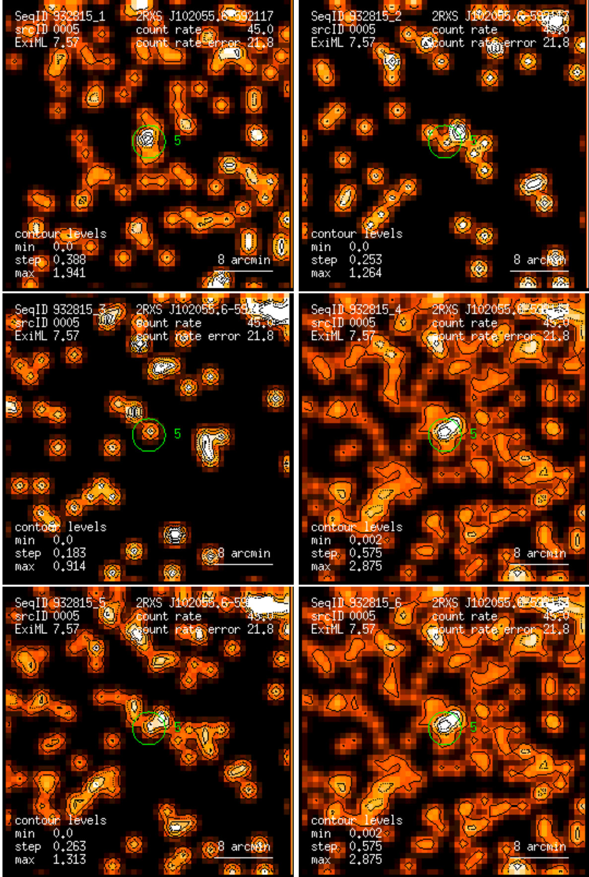
Figure 5: RASS 932815: detection 0005: band rate images, Gaussian filter: (1) PSPC channels 11 – 41, (2) 52 – 90, (3) 91 – 201, (4) 11 – 235, (5) 52 – 201, (6) 11 – 201. Broad band rates in counts/ks. Band rate contour levels in counts/ks/arcmin 2 .
