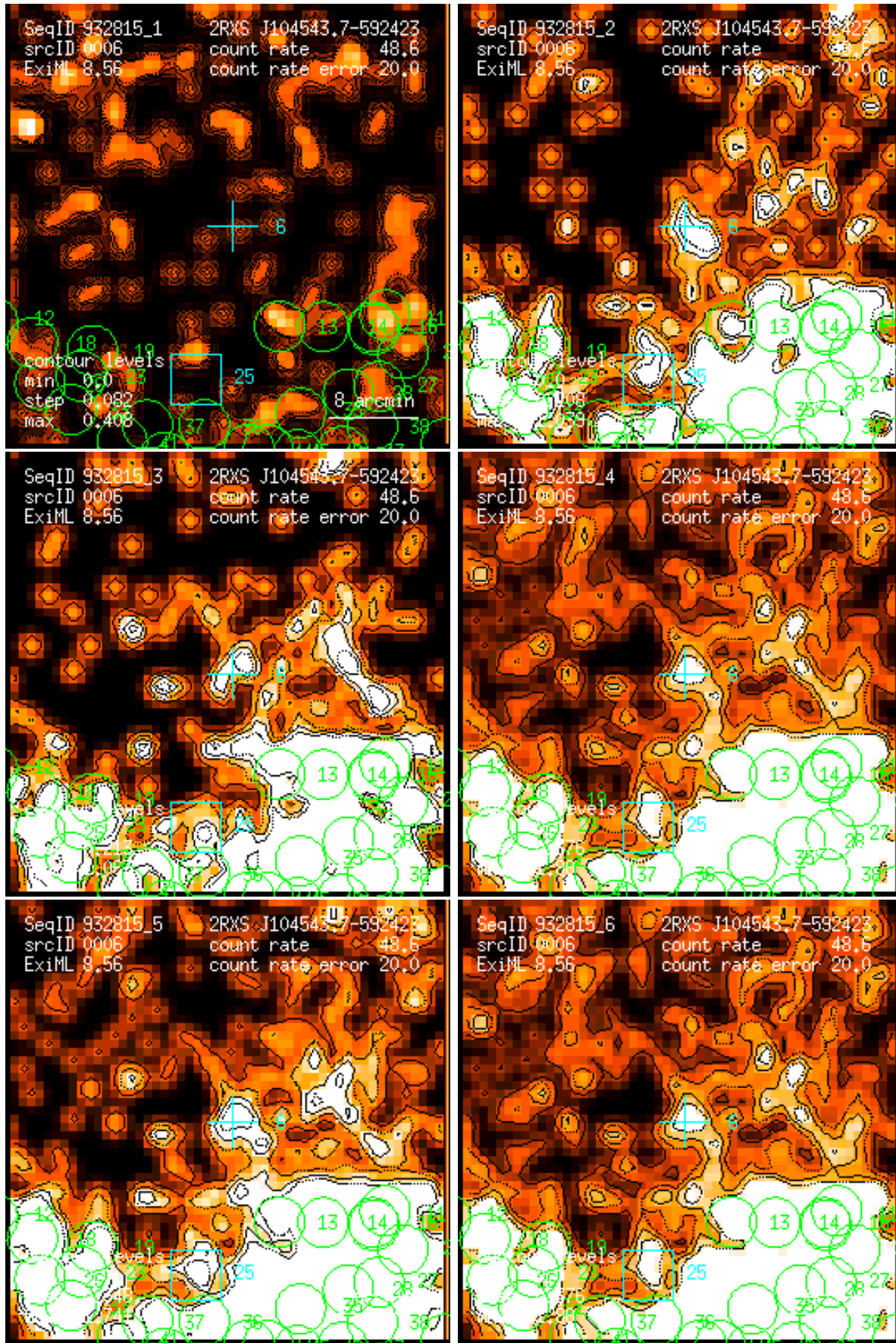
Figure 6: RASS 932815: detection 0006: band rate images, Gaussian filter: (1) PSPC channels 11 – 41, (2) 52 – 90, (3) 91 – 201, (4) 11 – 235, (5) 52 – 201, (6) 11 – 201. Broad band rates in counts/ks. Band rate contour levels in counts/ks/arcmin 2 .
