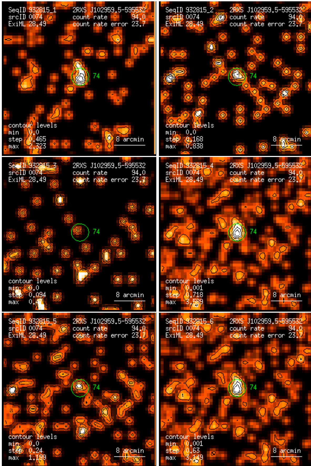
Figure 74: RASS 932815: detection 0074: band rate images, Gaussian filter: (1) PSPC channels 11 – 41, (2) 52 – 90, (3) 91 – 201, (4) 11 – 235, (5) 52 – 201, (6) 11 – 201. Broad band rates in counts/ks. Band rate contour levels in counts/ks/arcmin 2 .
