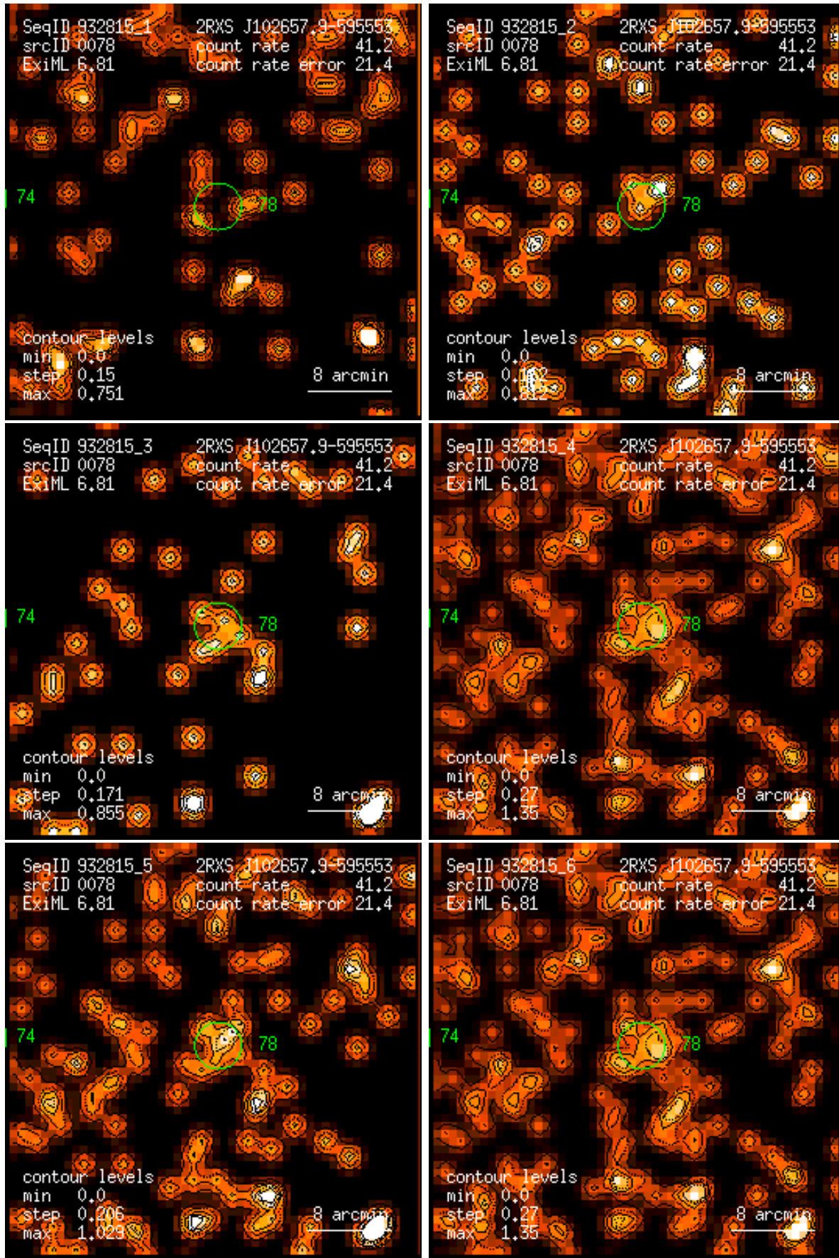
Figure 78: RASS 932815: detection 0078: band rate images, Gaussian filter: (1) PSPC channels 11 – 41, (2) 52 – 90, (3) 91 – 201, (4) 11 – 235, (5) 52 – 201, (6) 11 – 201. Broad band rates in counts/ks. Band rate contour levels in counts/ks/arcmin 2 .
